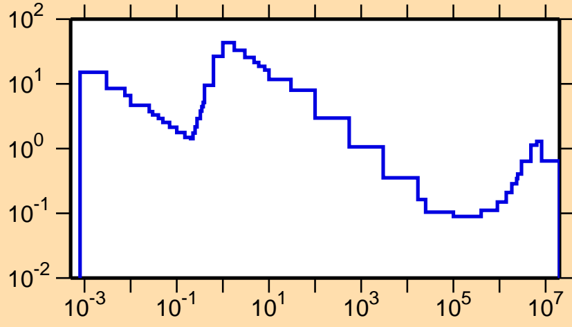
\sigma vs. E for ^{170}\text{Os}(n,p)
