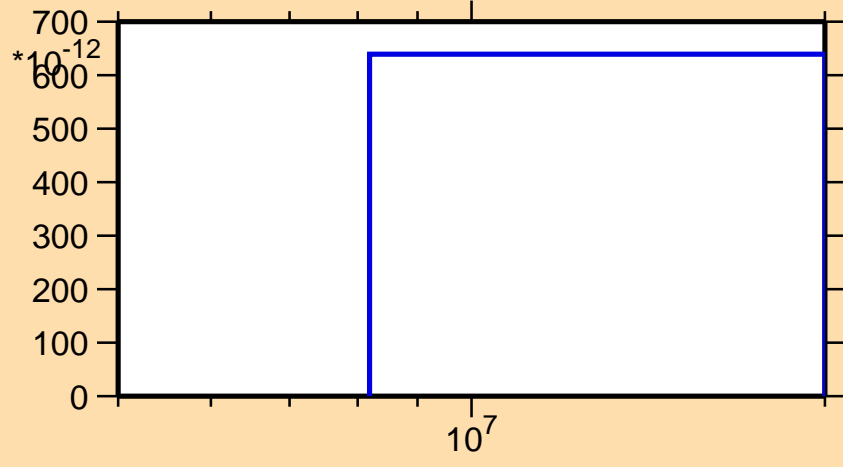
\sigma vs. E for ^{170}\text{Os}(n,pt)
