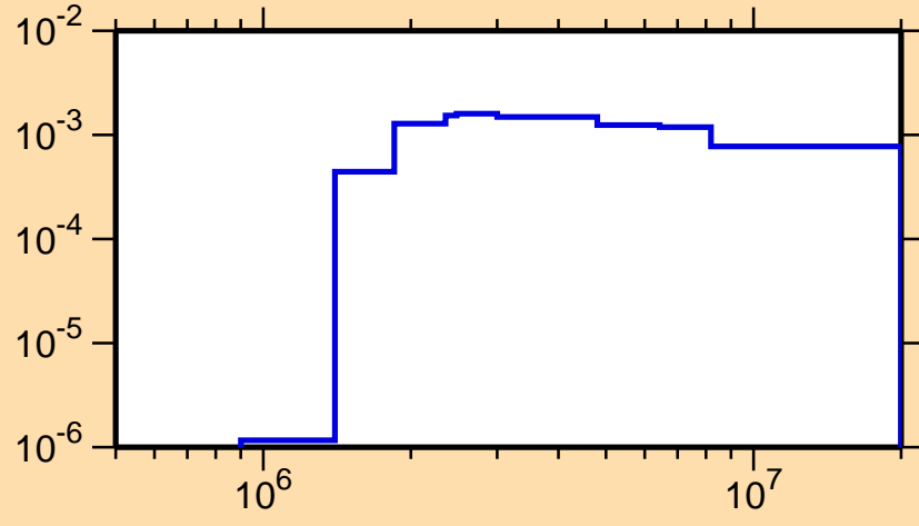
\sigma vs. E for ^{170}\text{Os}(n,n_3)
