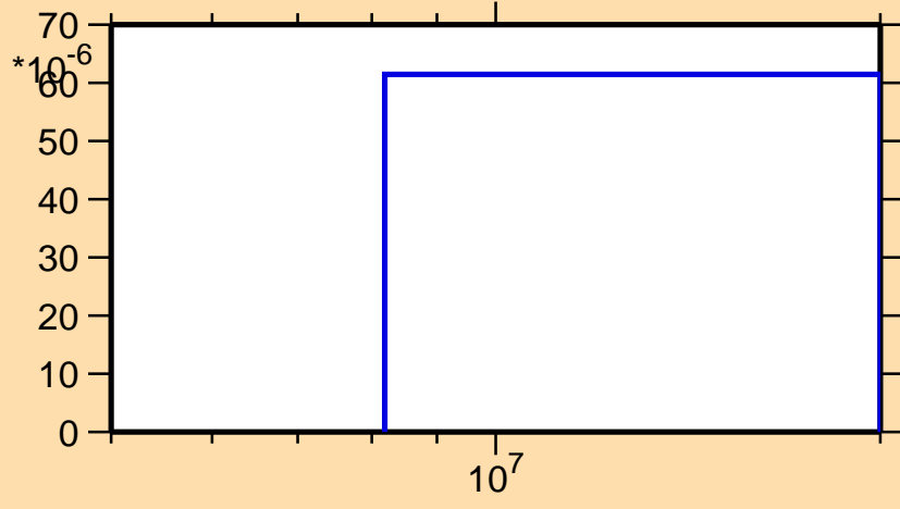
\sigma vs. E for ^{170}\text{Os}(n,t)
