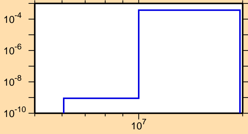
\sigma vs. E for ^{171}\text{Os}(n,t)
