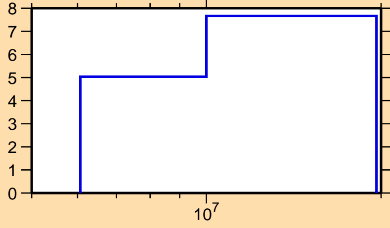
\Delta\sigma/\sigma vs. E for ^{171}\text{Os}(n,\text{nonel.})
