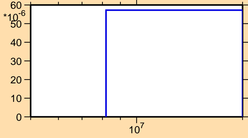
\sigma vs. E for ^{171}\text{Os}(n,2n\alpha)
