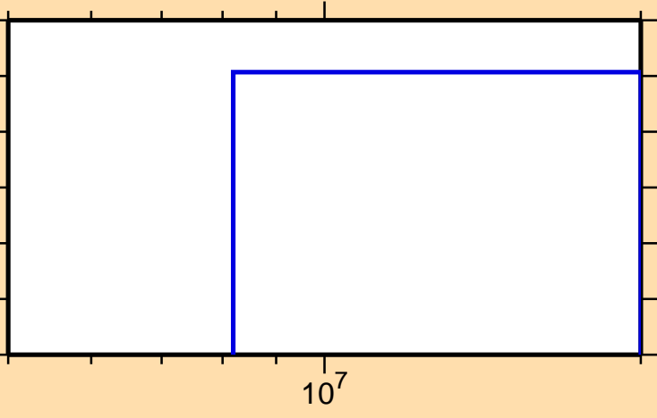
\sigma vs. E for ^{171}\text{Os}(n,2np)
