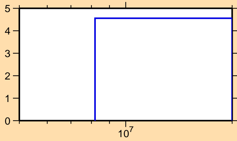
\Delta\sigma/\sigma vs. E for ^{171}\text{Os}(n,\text{tot.})
