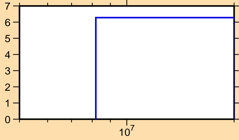
\Delta\sigma/\sigma vs. E for ^{171}\text{Os}(n,\text{el.})
