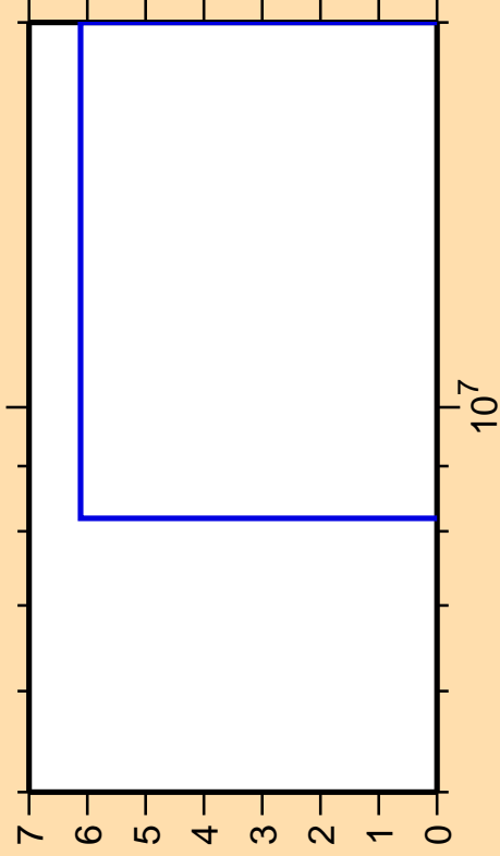
\Delta\sigma/\sigma vs. E for ^{171}\text{Os}(n,3n)
