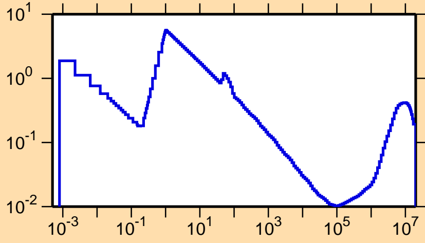
\sigma vs. E for ^{172}\text{Os}(n,p)
