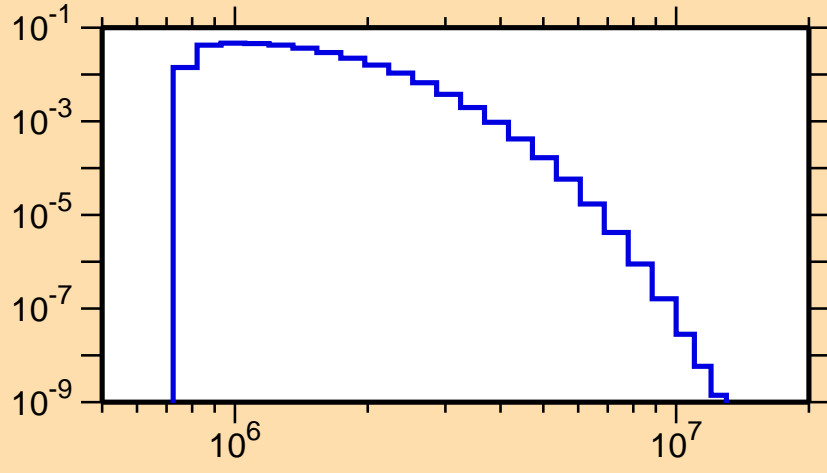
\sigma vs. E for ^{172}\text{Os}(n,n_4)
