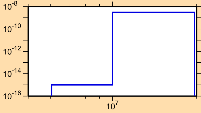
\sigma vs. E for ^{172}\text{Os}(\text{mt117})
