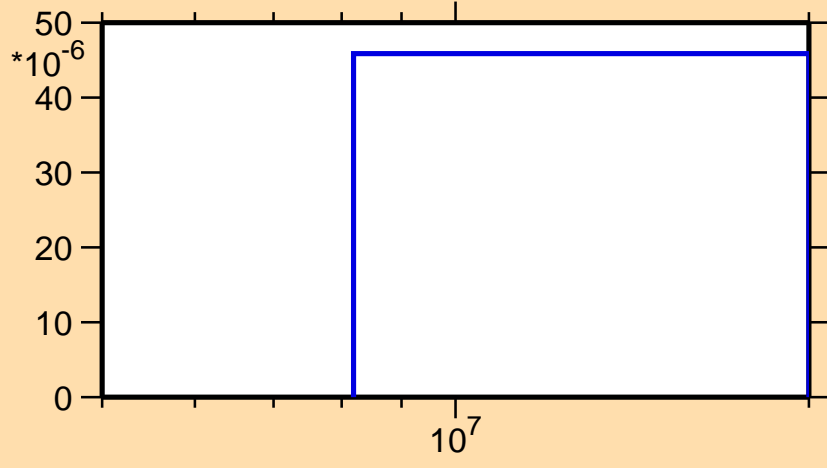
\sigma vs. E for ^{172}\text{Os}(n,t)
