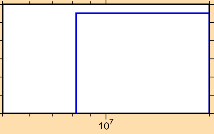
\sigma vs. E for ^{172}\text{Os}(n,2np)
