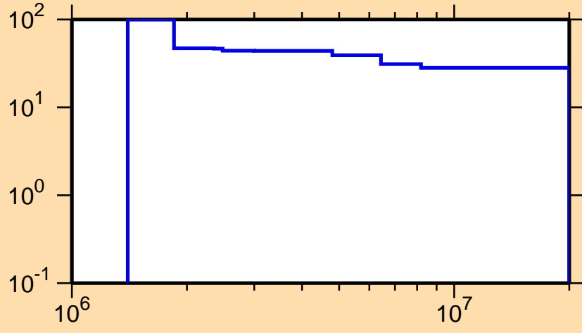
\Delta\sigma/\sigma vs. E for ^{172}\text{Os}(n,n\text{cont.})
