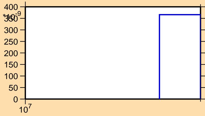
\sigma vs. E for ^{173}\text{Os}(n,3n)
