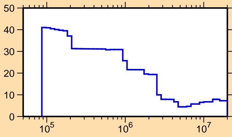
\Delta\sigma/\sigma vs. E for ^{173}\text{Os}(n,\text{nonel.})
