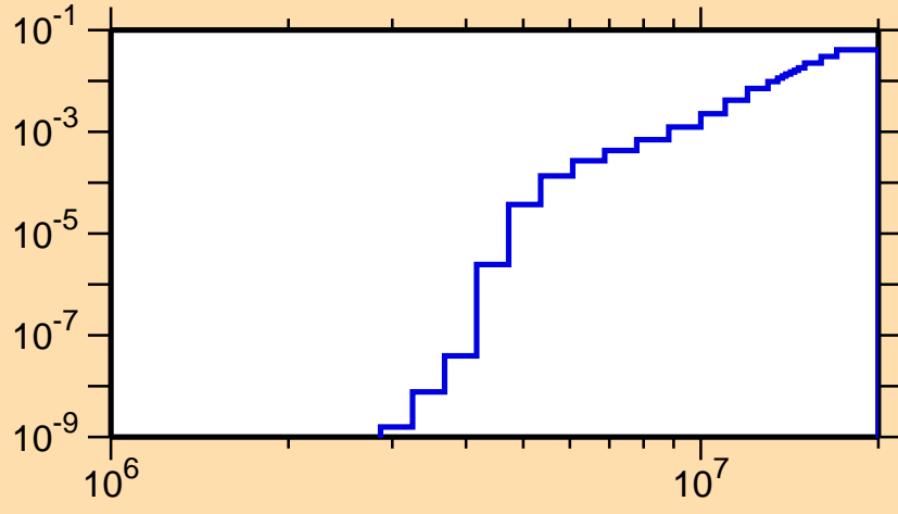
\sigma vs. E for ^{173}\text{Os}(n,n\alpha)
