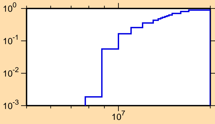
\sigma vs. E for ^{173}\text{Os}(n,2n)
