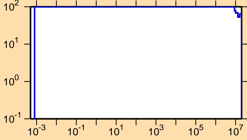
\Delta\sigma/\sigma vs. E for ^{173}\text{Os}(n,p)
