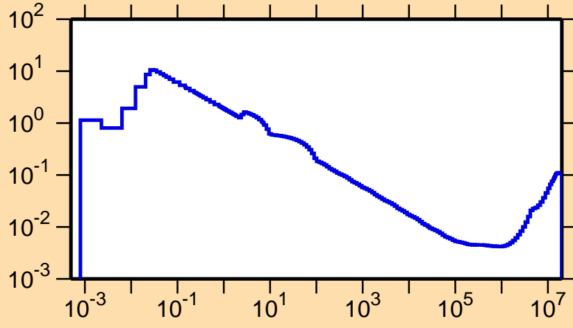
\sigma vs. E for ^{173}\text{Os}(n,\alpha)
