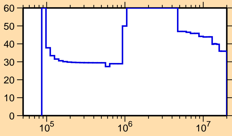
\Delta\sigma/\sigma vs. E for ^{173}\text{Os}(n,n_1)
