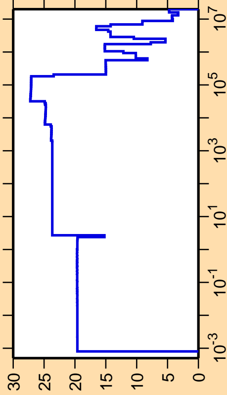
\Delta\sigma/\sigma vs. E for ^{173}\text{Os}(n,\text{el.})
