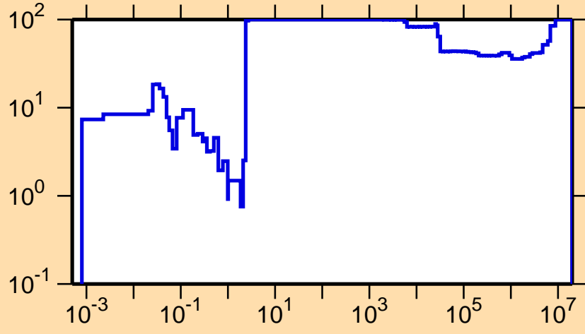
\Delta\sigma/\sigma vs. E for ^{173}\text{Os}(n,\gamma)
