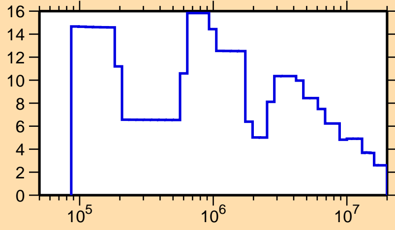
\Delta\sigma/\sigma vs. E for ^{173}\text{Os}(n,\text{tot.})
