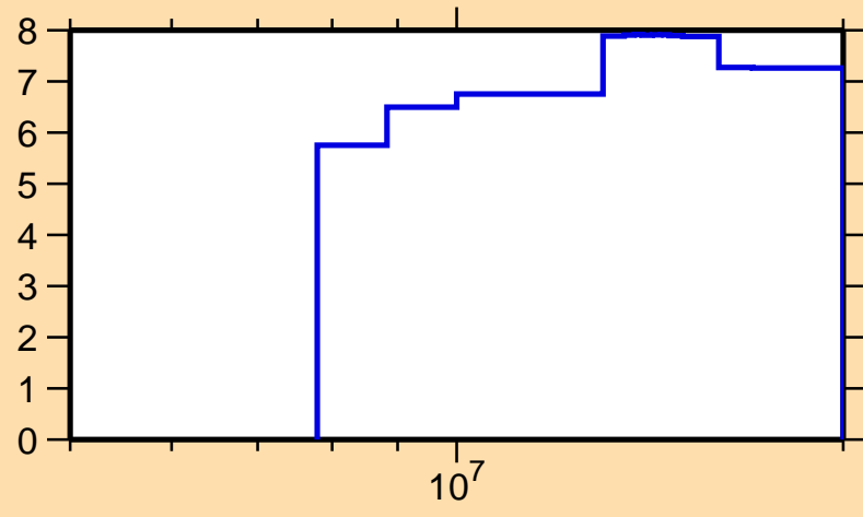
\Delta\sigma/\sigma vs. E for ^{173}\text{Os}(n,\text{nonel.})
