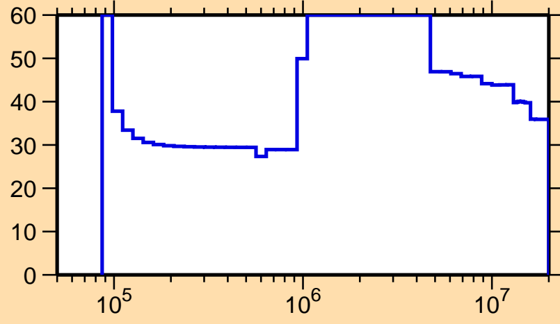
\Delta\sigma/\sigma vs. E for ^{173}\text{Os}(n,n_1)
