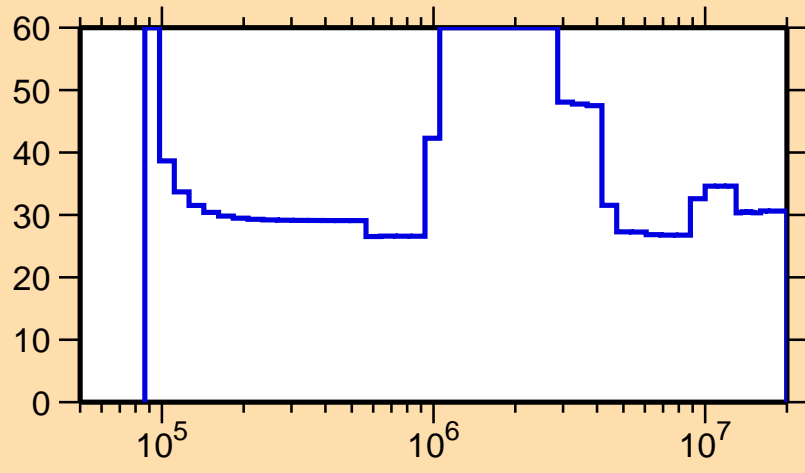
\Delta\sigma/\sigma vs. E for ^{173}\text{Os}(n,\text{inel.})
