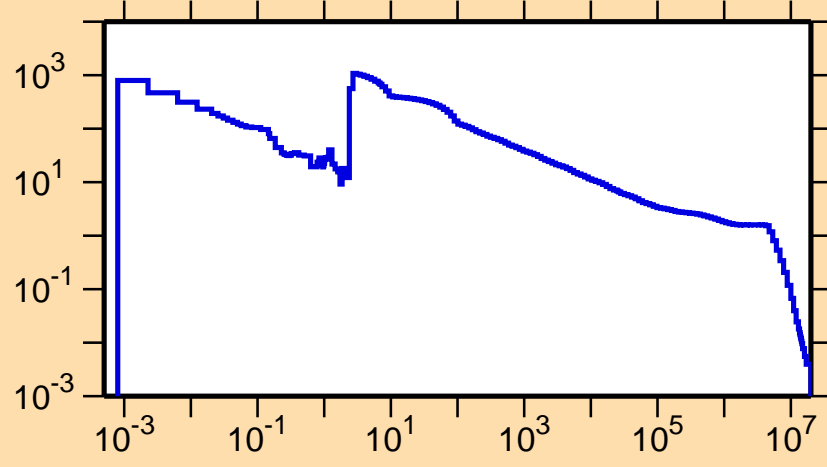
\sigma vs. E for ^{173}\text{Os}(n,\gamma)
