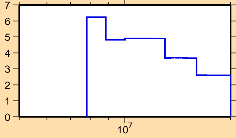
\Delta\sigma/\sigma vs. E for ^{173}\text{Os}(n,\text{tot.})
