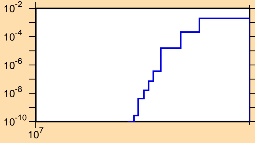
\sigma vs. E for ^{173}\text{Os}(n,2np)
