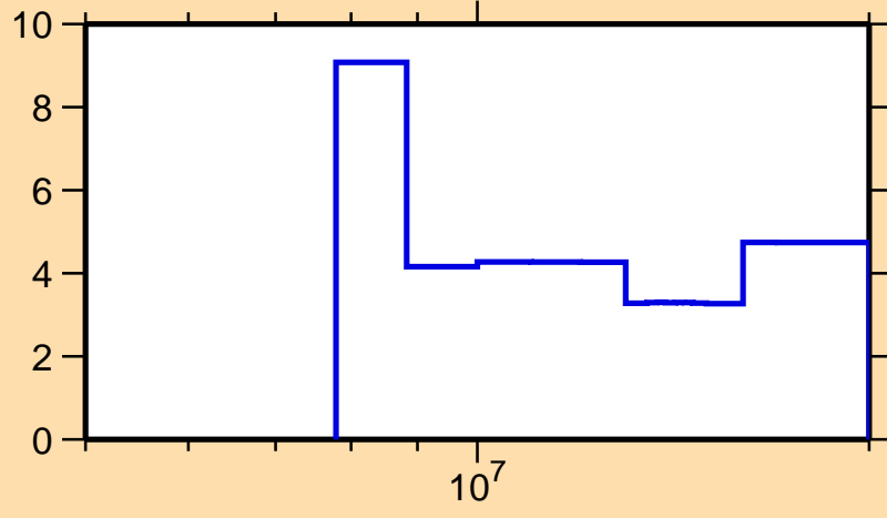
\Delta\sigma/\sigma vs. E for ^{173}\text{Os}(n,\text{el.})
