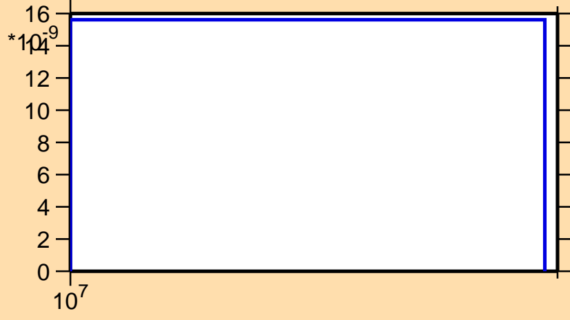
\sigma vs. E for ^{173}\text{Os}(n,\text{pt})
