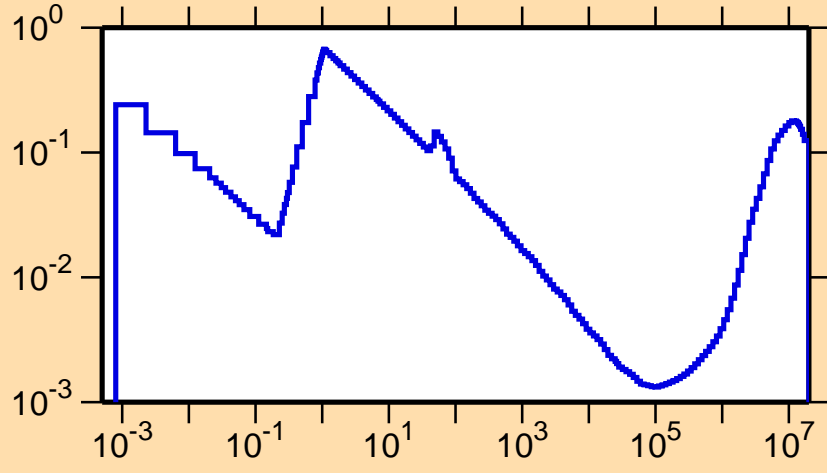
\sigma vs. E for ^{174}\text{Os}(n,p)
