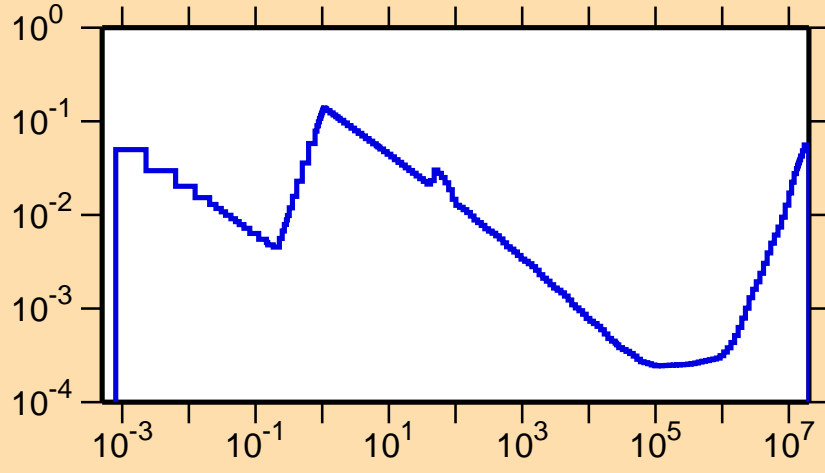
\sigma vs. E for ^{174}\text{Os}(n,\alpha)
