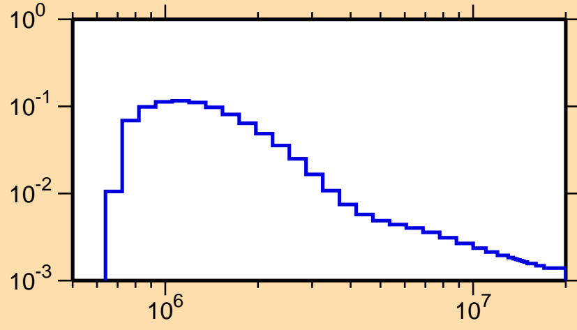
\sigma vs. E for ^{174}\text{Os}(n,n_4)
