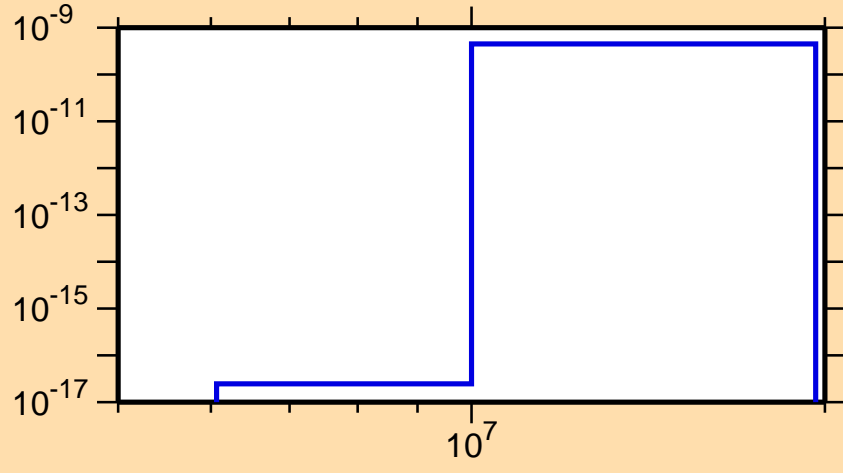
\sigma vs. E for ^{174}\text{Os}(\text{mt117})
