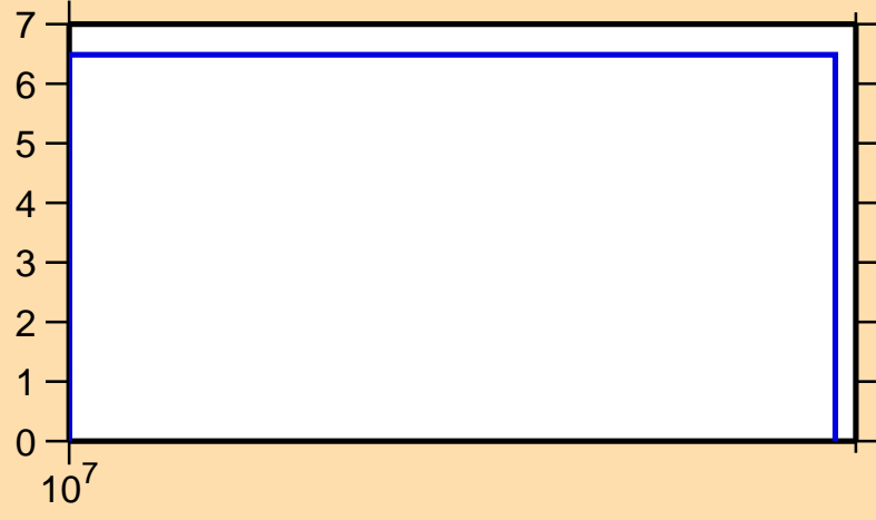
\Delta\sigma/\sigma vs. E for ^{174}\text{Os}(n,\text{el.})
