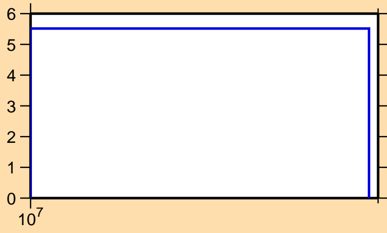
\Delta\sigma/\sigma vs. E for ^{174}\text{Os}(n,\text{tot.})
