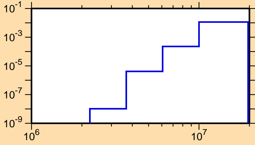
\sigma vs. E for ^{174}\text{Os}(n,n\alpha)
