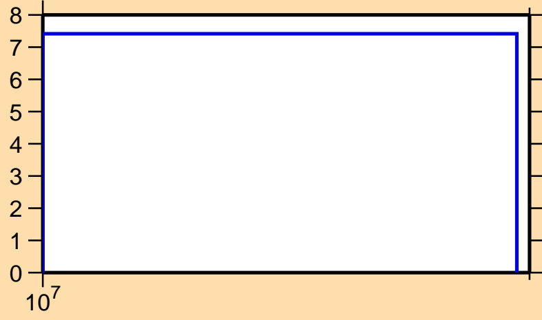
\Delta\sigma/\sigma vs. E for ^{174}\text{Os}(n,\text{nonel.})
