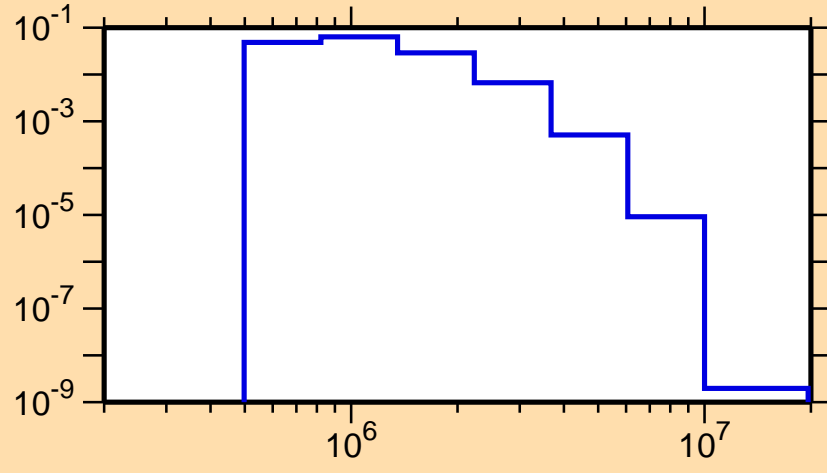
\sigma vs. E for ^{174}\text{Os}(n,n_3)
