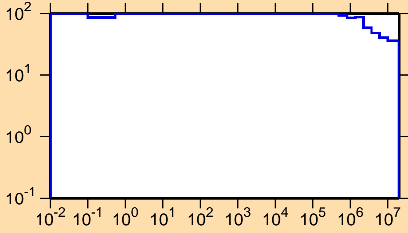
\Delta\sigma/\sigma vs. E for ^{174}\text{Os}(n,p)
