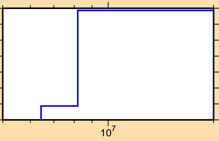
\sigma vs. E for ^{174}\text{Os}(n,\text{He}3)
