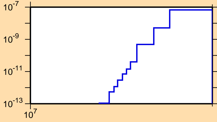
\sigma vs. E for ^{175}\text{Os}(n,\text{pt})
