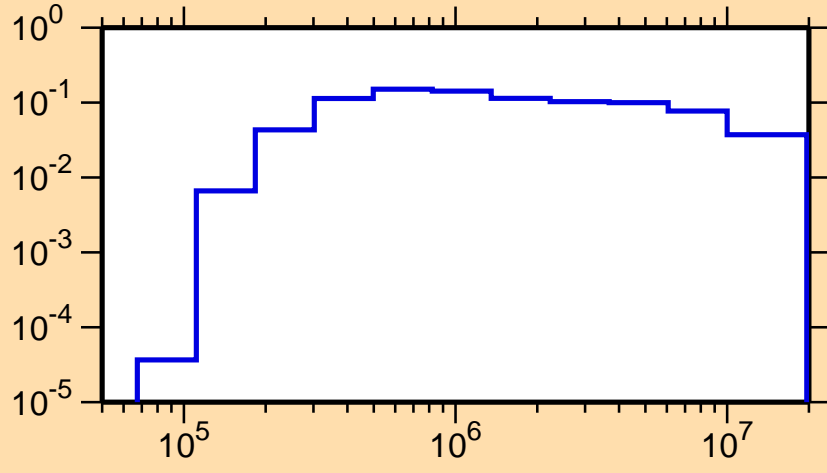
\sigma vs. E for ^{175}\text{Os}(n,n_3)
