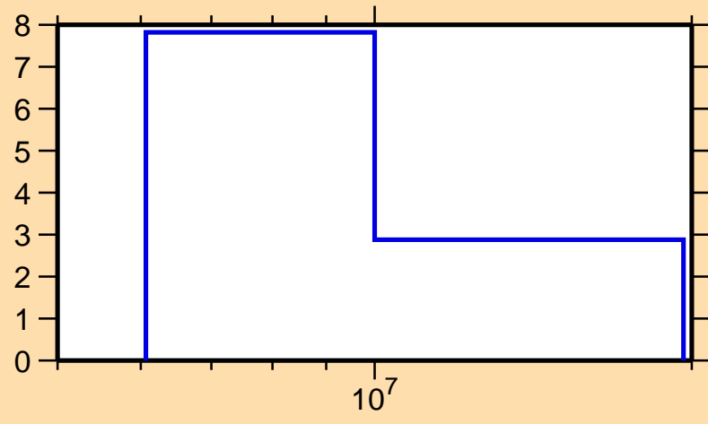
\Delta\sigma/\sigma vs. E for ^{175}\text{Os}(n,\text{tot.})
