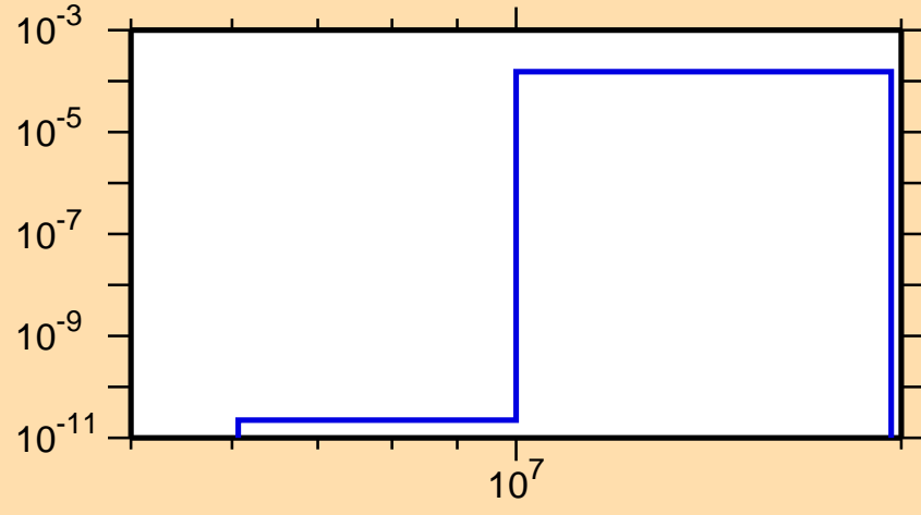
\sigma vs. E for ^{175}\text{Os}(n,t)
