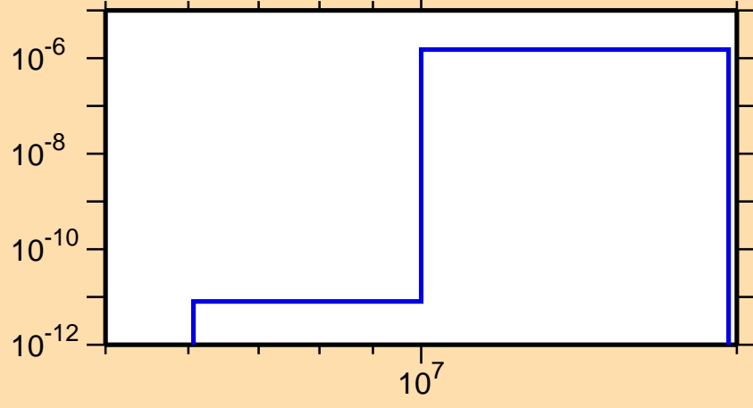
\sigma vs. E for ^{175}\text{Os}(n,\text{He}3)
