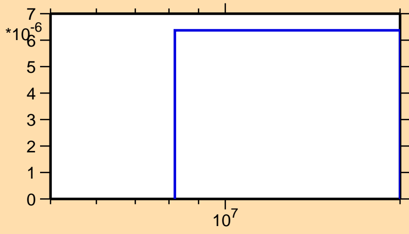
\sigma vs. E for ^{175}\text{Os}(n,2n\alpha)
