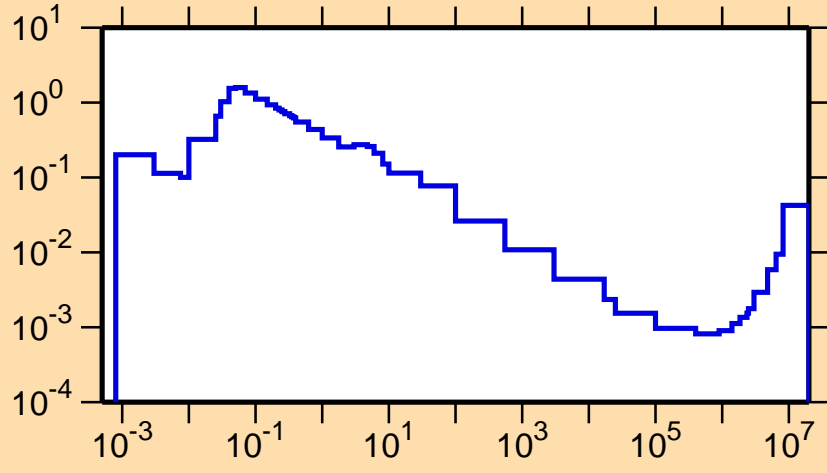
\sigma vs. E for ^{175}\text{Os}(n,\alpha)
