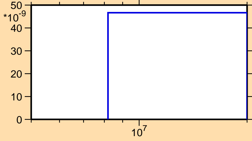
\sigma vs. E for ^{175}\text{Os}(n,\text{nd})
