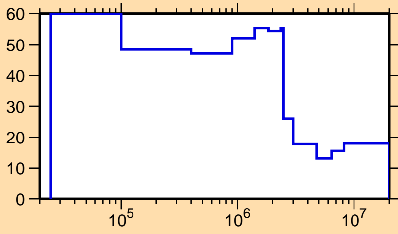
\Delta\sigma/\sigma vs. E for ^{175}\text{Os}(n,n_1)
