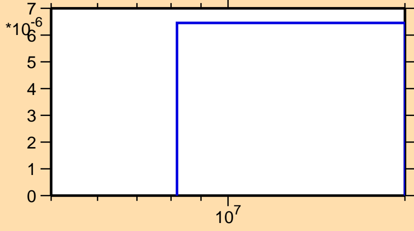
\sigma vs. E for ^{175}\text{Os}(n,2np)
