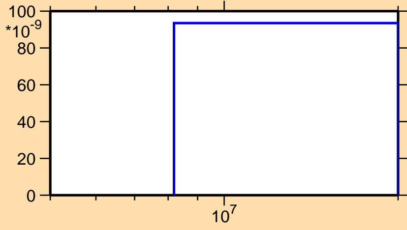
\sigma vs. E for ^{175}\text{Os}(n,3n)
