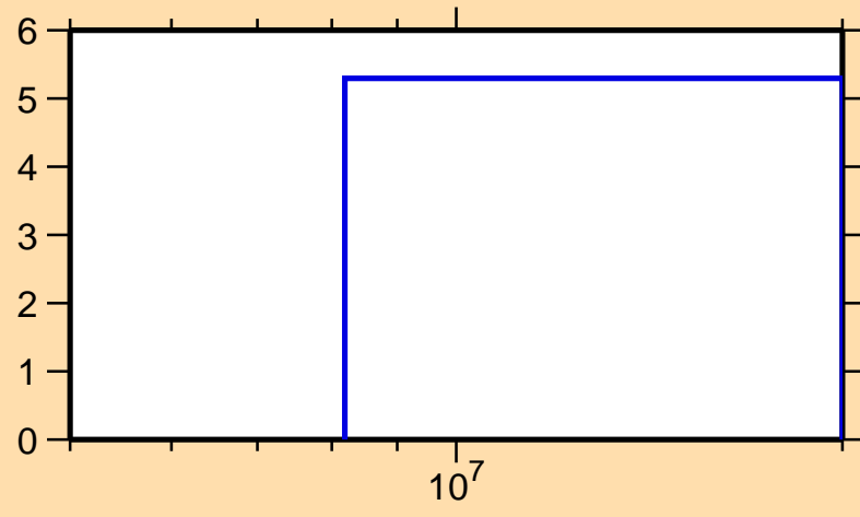
\Delta\sigma/\sigma vs. E for ^{175}\text{Os}(n,\text{el.})
