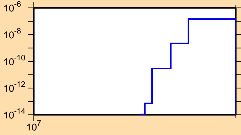
\sigma vs. E for ^{176}\text{Os}(n,\text{nd})
