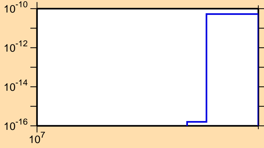
\sigma vs. E for ^{176}\text{Os}(n,nt)
