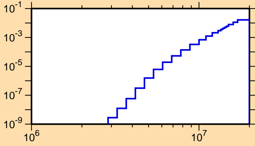
\sigma vs. E for ^{176}\text{Os}(n,n\alpha)
