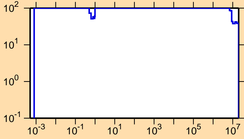
\Delta\sigma/\sigma vs. E for ^{176}\text{Os}(n,p)
