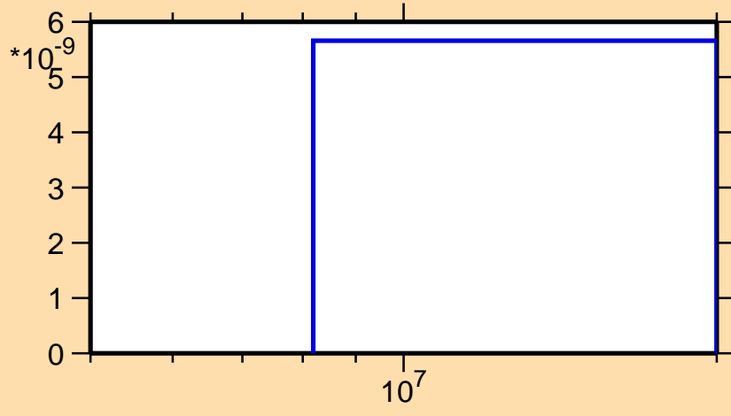
\sigma vs. E for ^{176}\text{Os} (mt 45)
