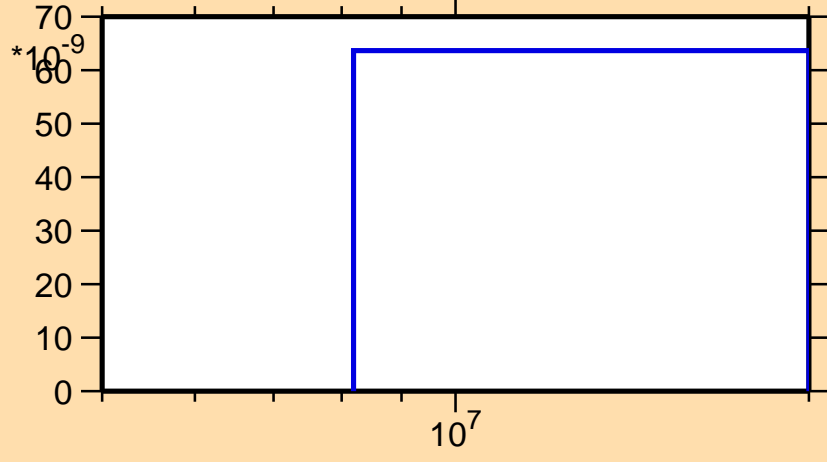
\sigma vs. E for ^{176}\text{Os}(n,2np)
