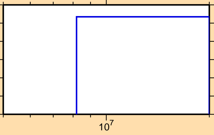
\sigma vs. E for ^{176}\text{Os}(n,\text{pd})
