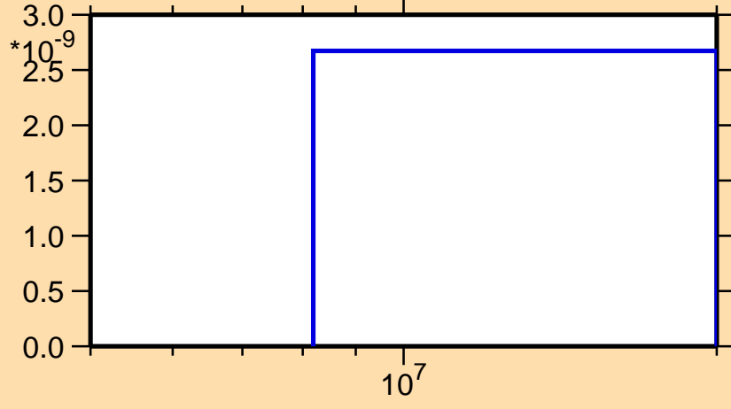
\sigma vs. E for ^{176}\text{Os}(n,\text{pd})
