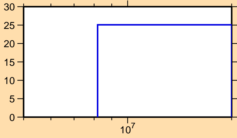
\Delta\sigma/\sigma vs. E for ^{176}\text{Os}(n,\text{inel.})
