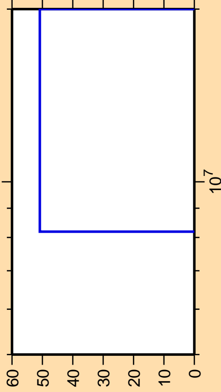
\Delta\sigma/\sigma vs. E for ^{176}\text{Os}(n,n_1)
