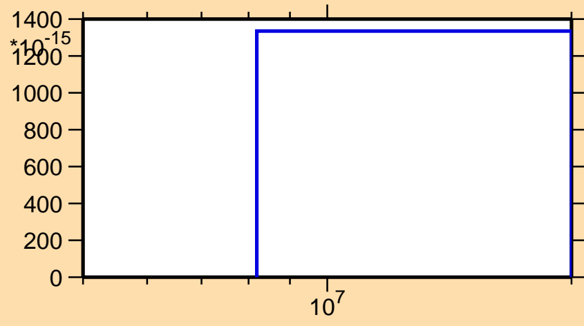
\sigma vs. E for ^{176}\text{Os}(n,pt)
