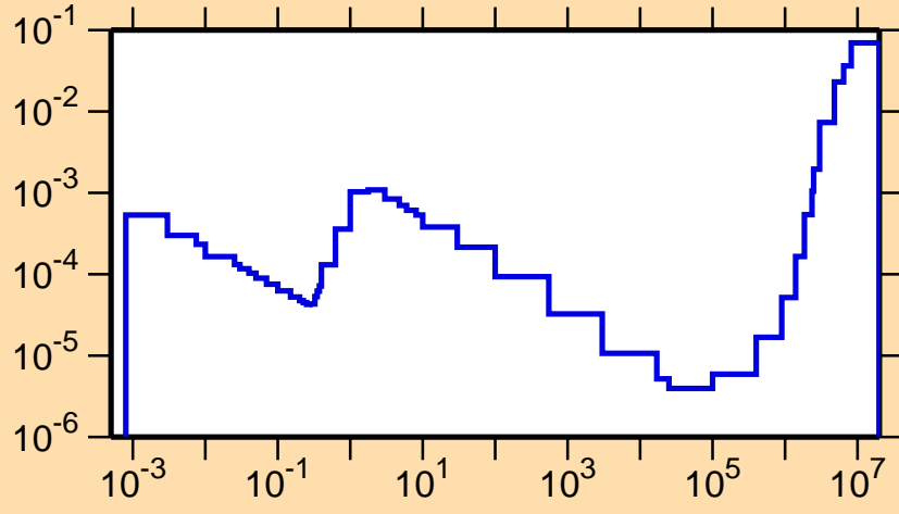
\sigma vs. E for ^{176}\text{Os}(n,p)
