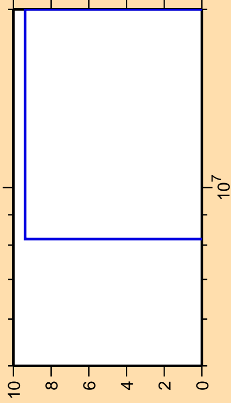
\Delta\sigma/\sigma vs. E for ^{176}\text{Os}(n,pt)
