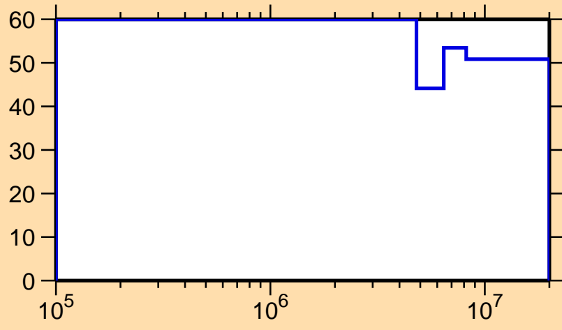
\Delta\sigma/\sigma vs. E for ^{176}\text{Os}(n,n_1)
