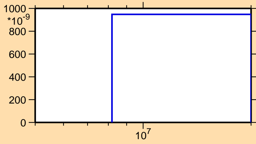
\sigma vs. E for ^{176}\text{Os}(n,3n)
