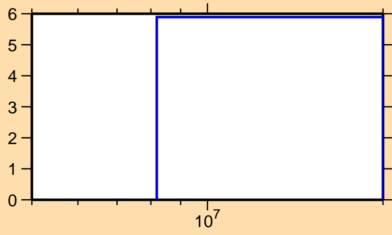
\Delta\sigma/\sigma vs. E for ^{176}\text{Os}(n,\text{el.})
