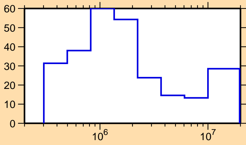
\Delta\sigma/\sigma vs. E for ^{177}\text{Os}(n,n\text{cont.})
