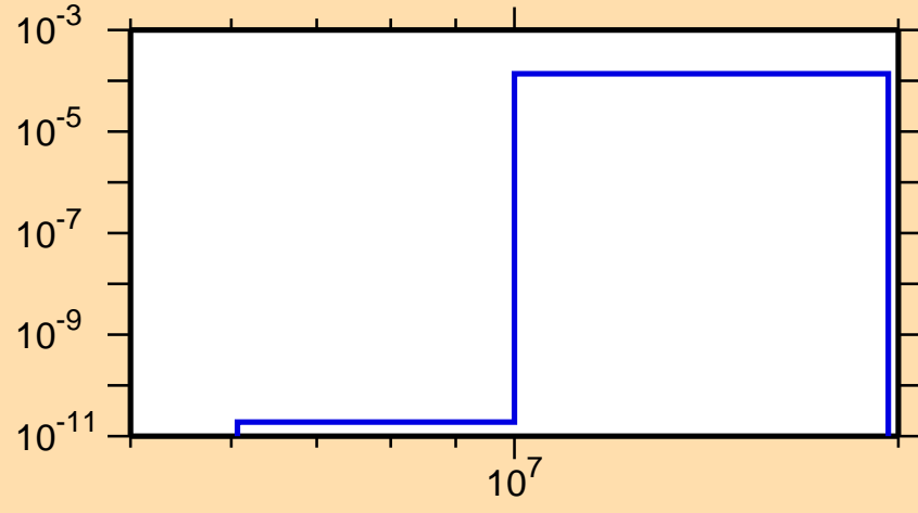
\sigma vs. E for ^{177}\text{Os}(n,t)
