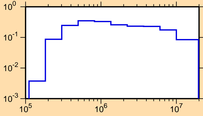
\sigma vs. E for ^{177}\text{Os}(n,n_3)
