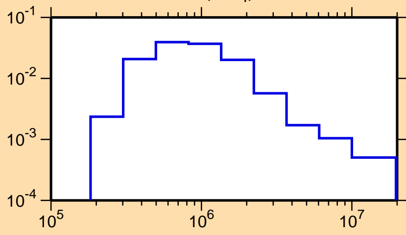
\sigma vs. E for ^{177}\text{Os}(n,n_4)
