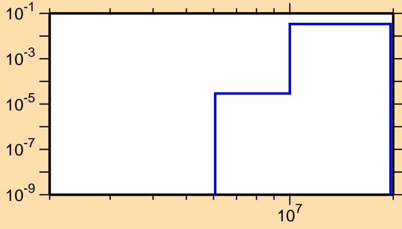
\sigma vs. E for ^{177}\text{Os}(n,np)
