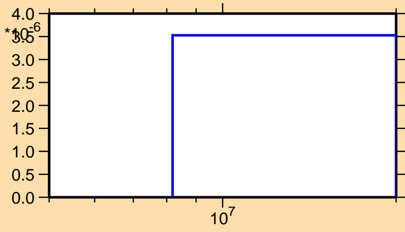
\sigma vs. E for ^{177}\text{Os}(n,3n)
