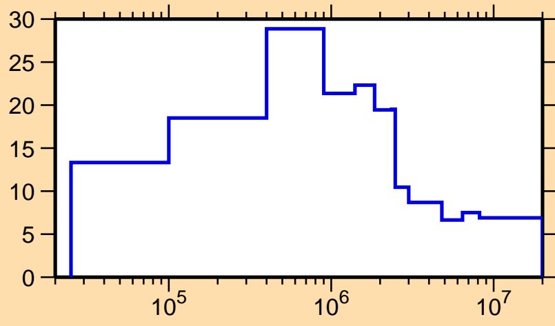
\Delta\sigma/\sigma vs. E for ^{177}\text{Os}(n,\text{nonel.})
