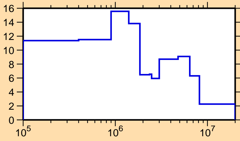
\Delta\sigma/\sigma vs. E for ^{177}\text{Os}(n,\text{tot.})
