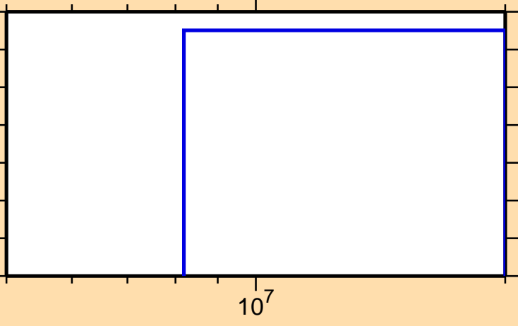
\sigma vs. E for ^{177}\text{Os}(n,\text{He}3)
