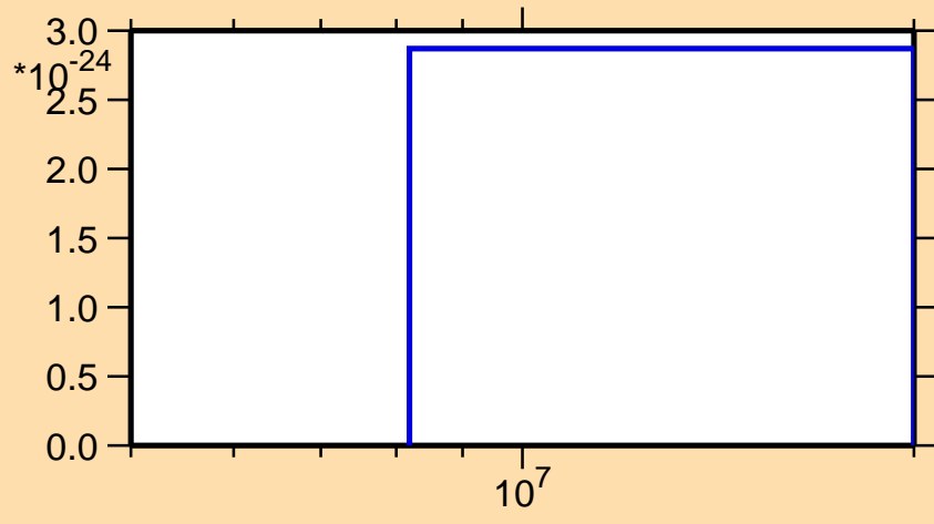
\sigma vs. E for ^{177}\text{Os} (mt 11)
