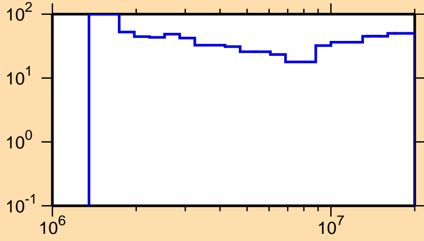
\Delta\sigma/\sigma vs. E for ^{178}\text{Os}(n,n\text{cont.})
