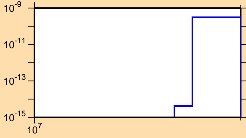
\sigma vs. E for ^{178}\text{Os}(n,nt)
