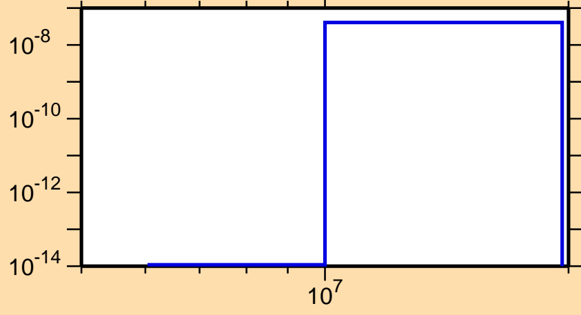
\sigma vs. E for ^{178}\text{Os}(n,\text{He}3)
