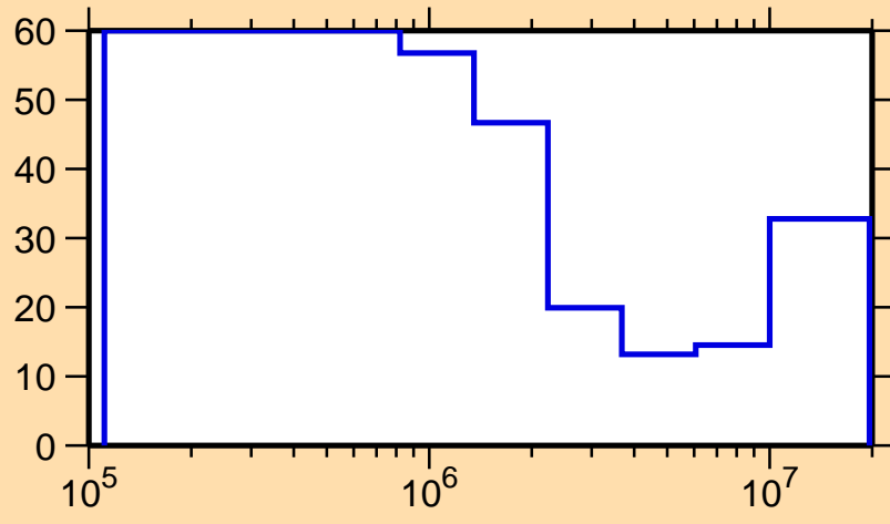
\Delta\sigma/\sigma vs. E for ^{178}\text{Os}(n,\text{inel.})
