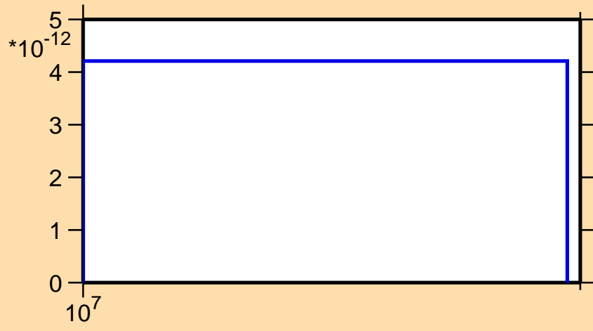
\sigma vs. E for ^{178}\text{Os}(\text{mt117})
