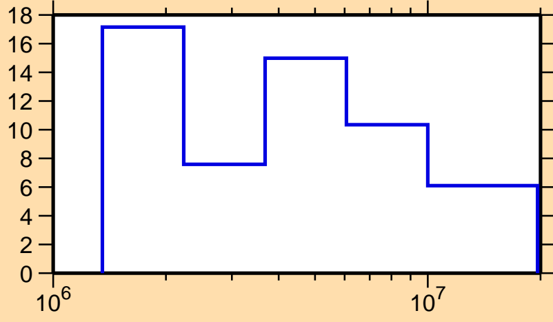
\Delta\sigma/\sigma vs. E for ^{178}\text{Os}(n,\text{el.})
