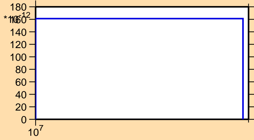
\sigma vs. E for ^{178}\text{Os} (mt 45)
