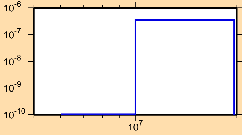
\sigma vs. E for ^{178}\text{Os}(n,p\alpha)
