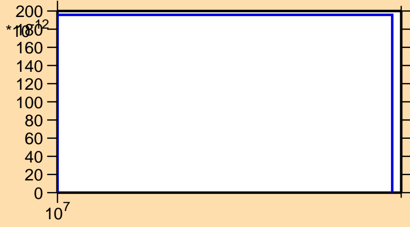
\sigma vs. E for ^{178}\text{Os}(n,pd)
