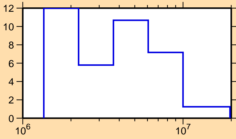
\Delta\sigma/\sigma vs. E for ^{178}\text{Os}(n,\text{tot.})
