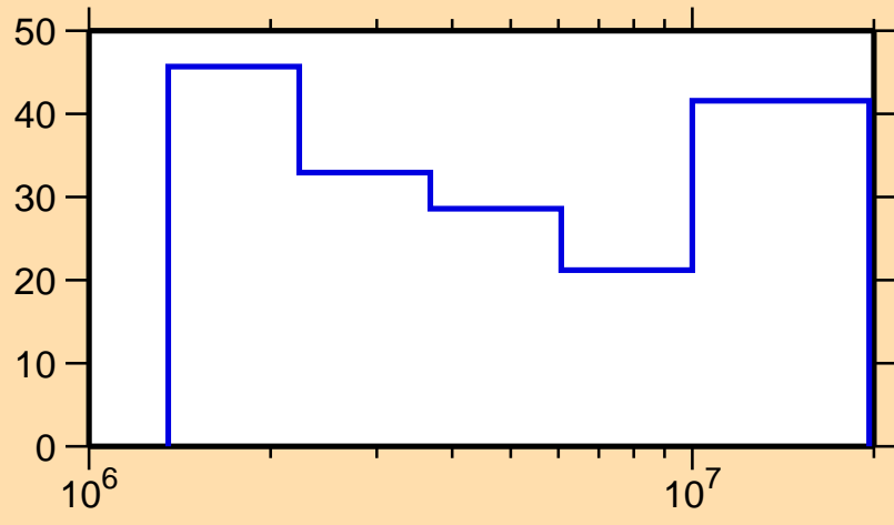
\Delta\sigma/\sigma vs. E for ^{178}\text{Os}(n,n\text{cont.})
