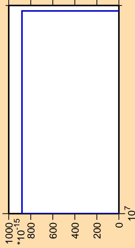
\Delta\sigma/\sigma vs. E for ^{178}\text{Os} (mt 11)
