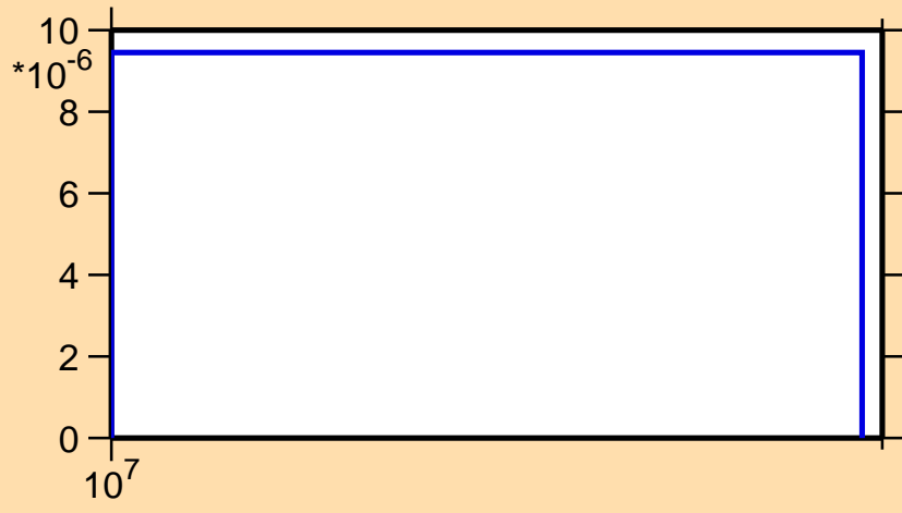
\sigma vs. E for ^{178}\text{Os}(n,3n)
