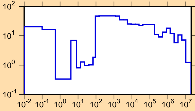
\Delta\sigma/\sigma vs. E for ^{178}\text{Os}(n,\text{tot.})
