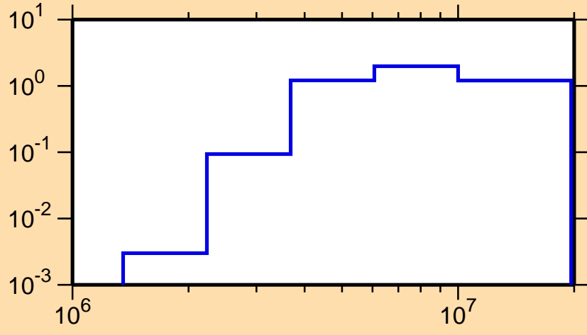
\sigma vs. E for ^{178}\text{Os}(n,n\text{cont.})
