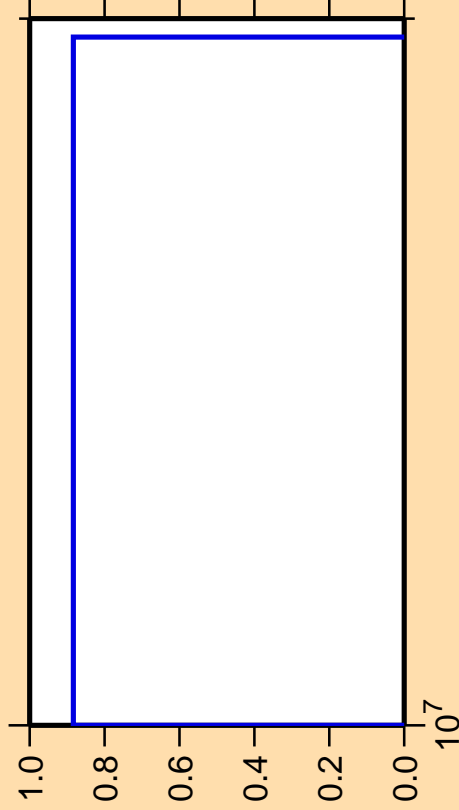
\Delta\sigma/\sigma vs. E for ^{178}\text{Os}(n,\text{pt})
