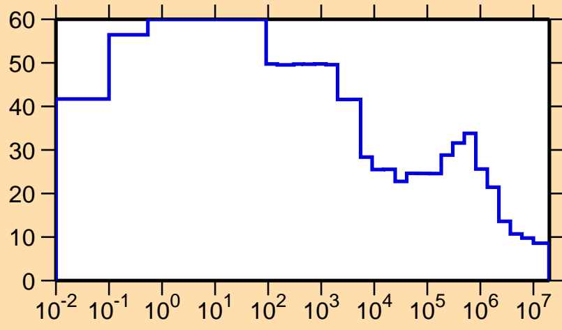
\Delta\sigma/\sigma vs. E for ^{178}\text{Os}(n,\text{nonel.})
