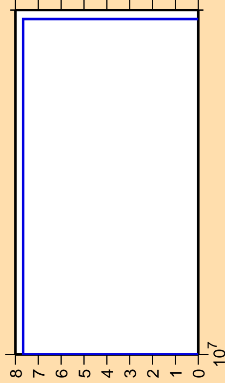
\Delta\sigma/\sigma vs. E for ^{178}\text{Os}(n,nt)
