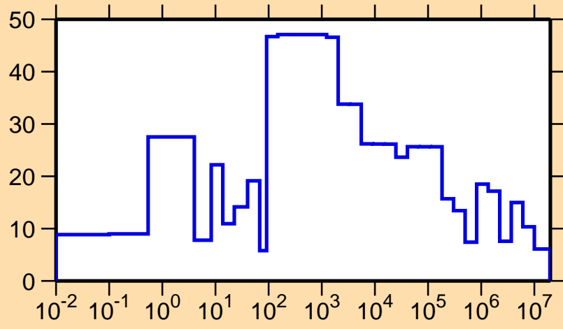
\Delta\sigma/\sigma vs. E for ^{178}\text{Os}(n,\text{el.})
