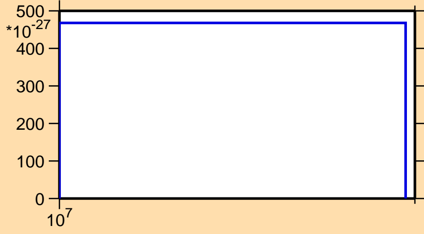
\sigma vs. E for ^{178}\text{Os} (mt 11)
