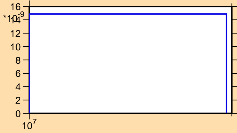
\sigma vs. E for ^{178}\text{Os}(n,2np)
