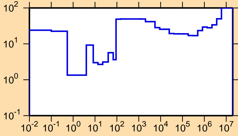
\Delta\sigma/\sigma vs. E for ^{178}\text{Os}(n,\gamma)
