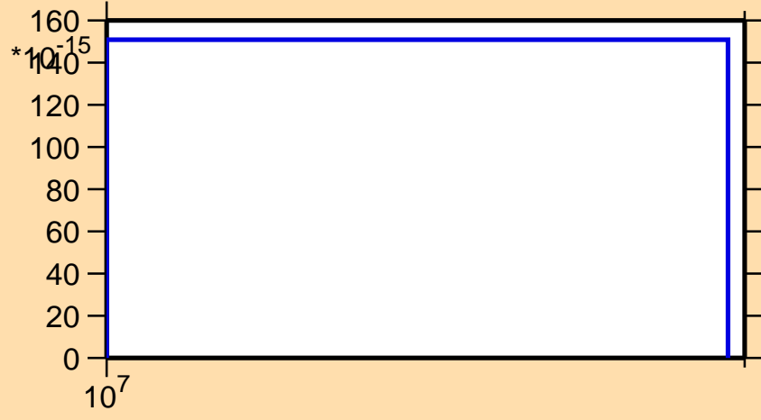
\sigma vs. E for ^{178}\text{Os}(n,\text{pt})
