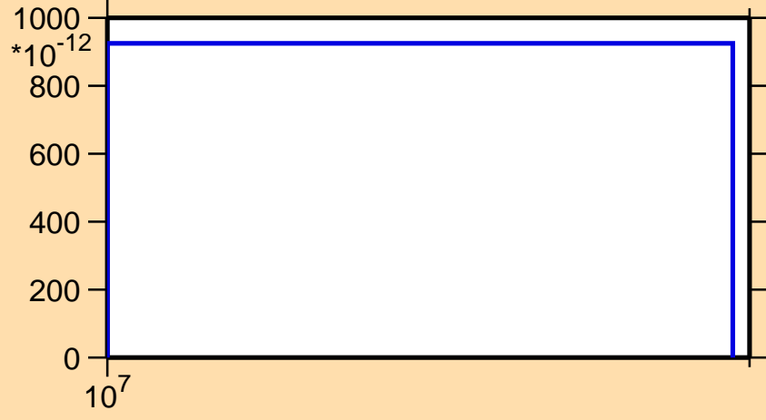
\sigma vs. E for ^{178}\text{Os}(n,\text{nd})
