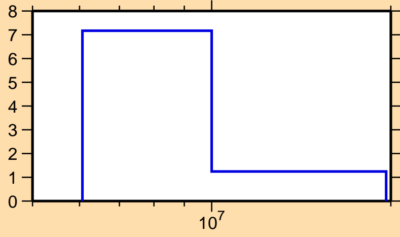
\Delta\sigma/\sigma vs. E for ^{178}\text{Os}(n,\text{tot.})
