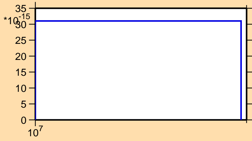
\sigma vs. E for ^{178}\text{Os} (mt 34)
