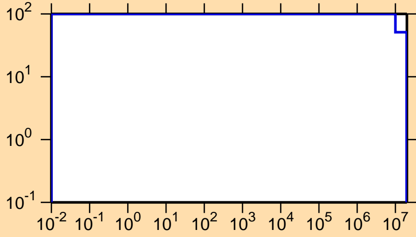
\Delta\sigma/\sigma vs. E for ^{178}\text{Os}(n,p)
