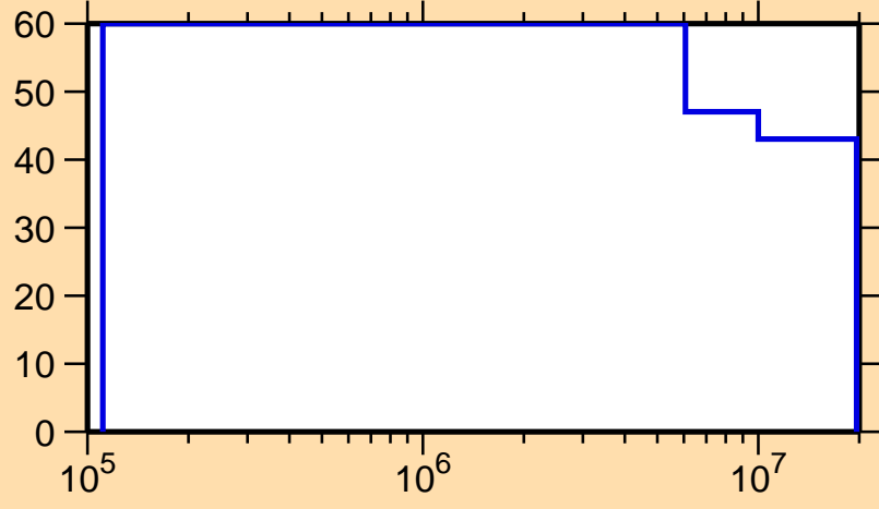
\Delta\sigma/\sigma vs. E for ^{178}\text{Os}(n,n_1)
