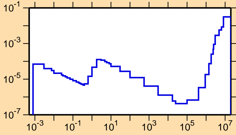
\sigma vs. E for ^{178}\text{Os}(n,p)
