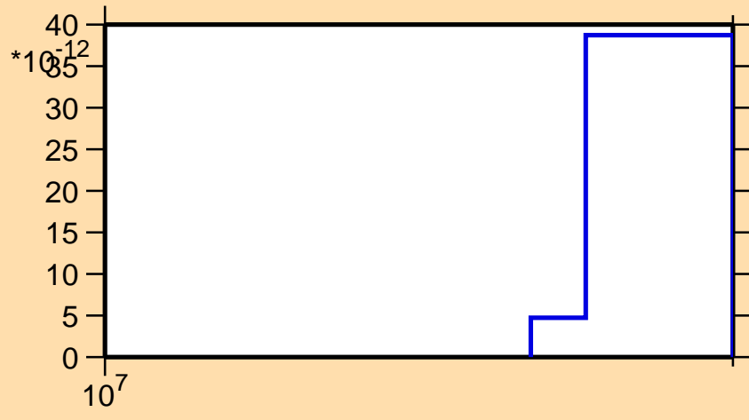
\sigma vs. E for ^{179}\text{Os}(\text{mt117})
