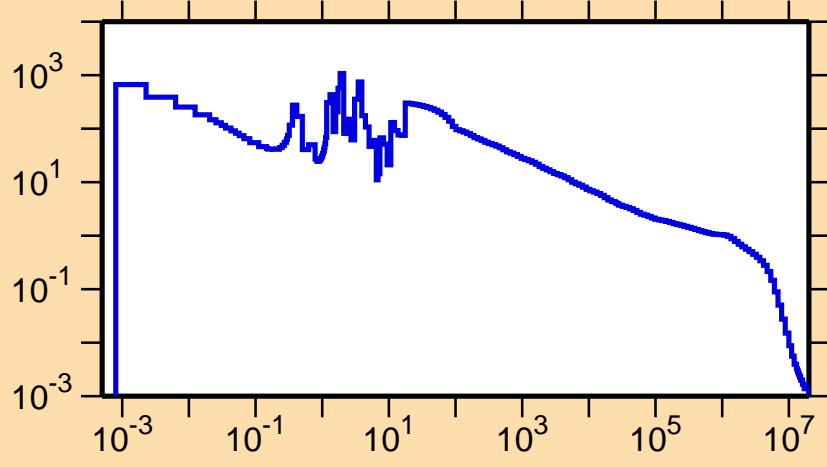
\sigma vs. E for ^{179}\text{Os}(n,\gamma)
