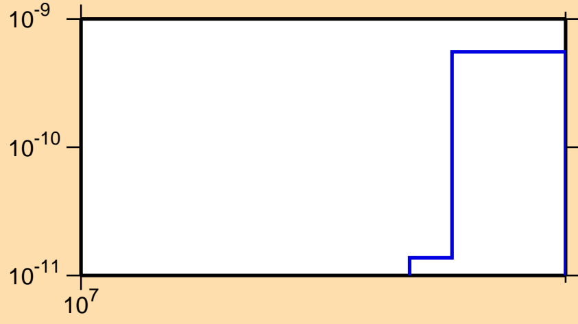
\sigma vs. E for ^{179}\text{Os}(n,\text{pt})
