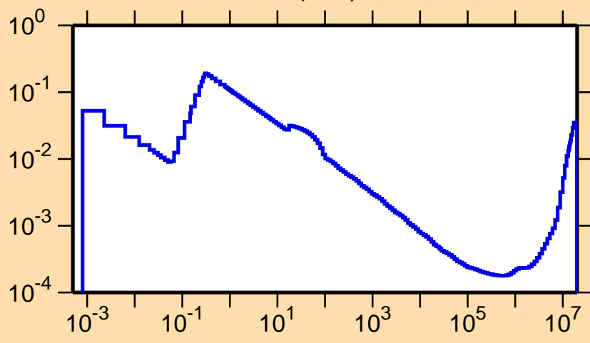
\sigma vs. E for ^{179}\text{Os}(n,\alpha)
