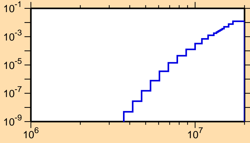
\sigma vs. E for ^{179}\text{Os}(n,n\alpha)
