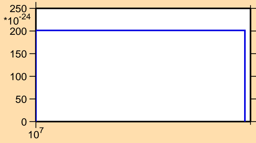
\sigma vs. E for ^{179}\text{Os} (mt 11)
