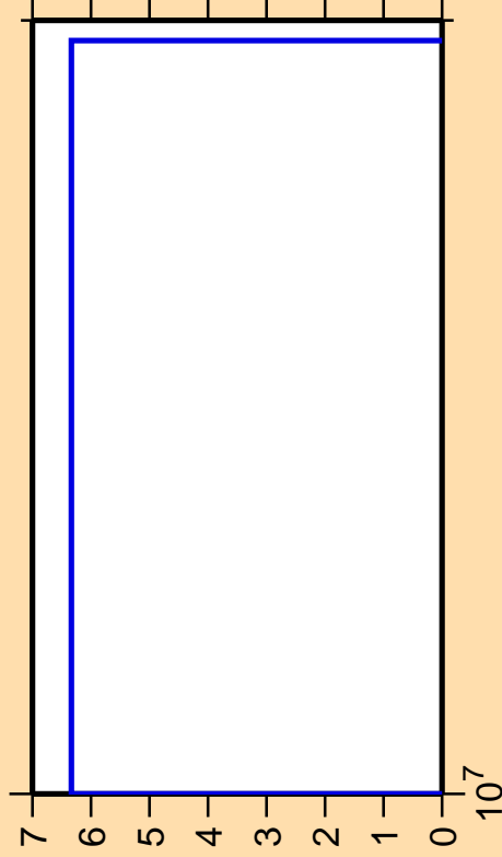
\Delta\sigma/\sigma vs. E for ^{179}\text{Os}(n,nt)
