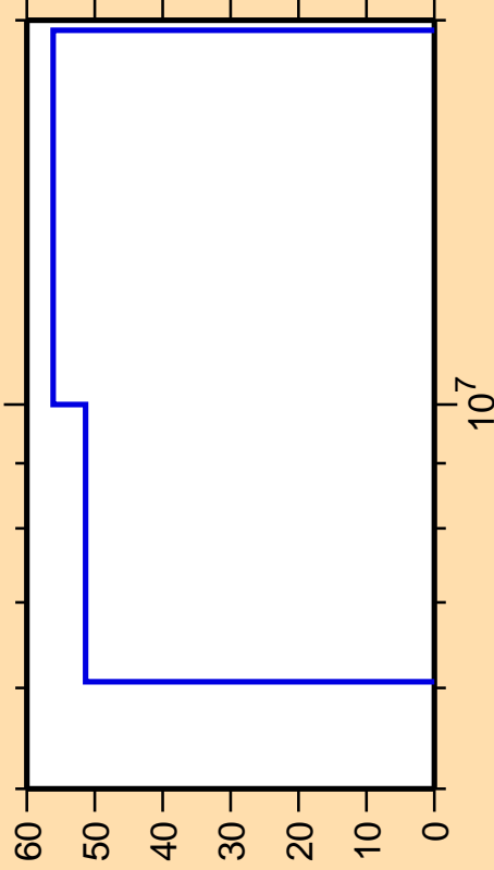
\Delta\sigma/\sigma vs. E for ^{179}\text{Os}(n,\gamma)
