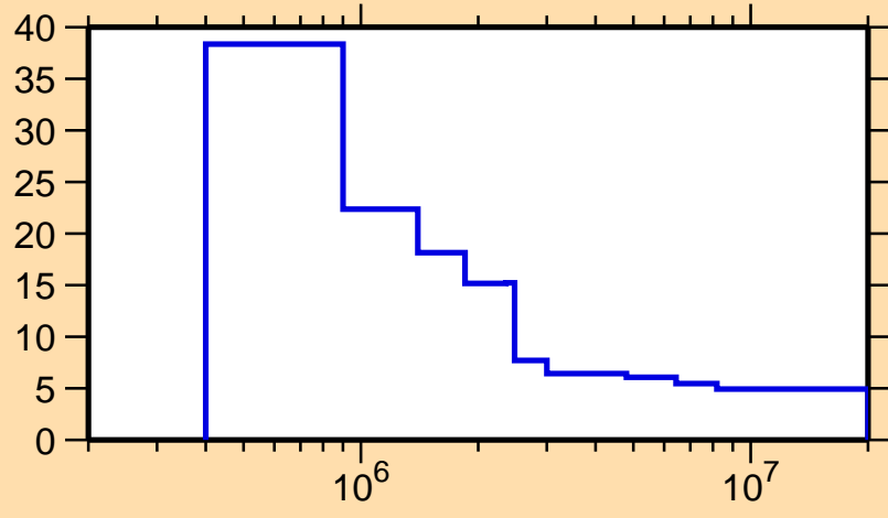
\Delta\sigma/\sigma vs. E for ^{179}\text{Os}(n,n\text{onel.})
