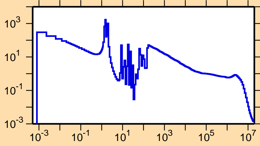
\sigma vs. E for ^{180}\text{Os}(n,\gamma)
