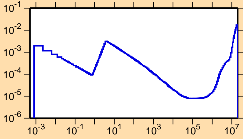
\sigma vs. E for ^{180}\text{Os}(n,\alpha)
