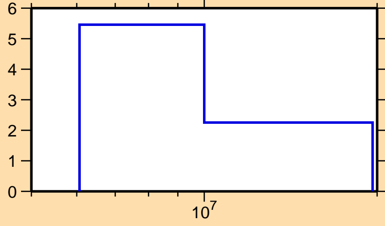
\Delta\sigma/\sigma vs. E for ^{180}\text{Os}(n,\text{el.})
