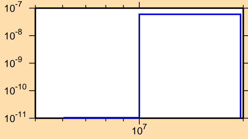
\sigma vs. E for ^{180}\text{Os}(n,p\alpha)
