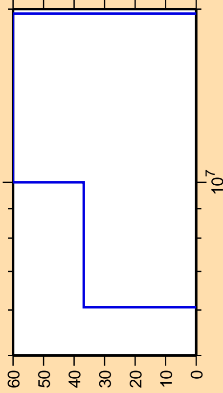
\Delta\sigma/\sigma vs. E for ^{180}\text{Os}(n,p\alpha)
