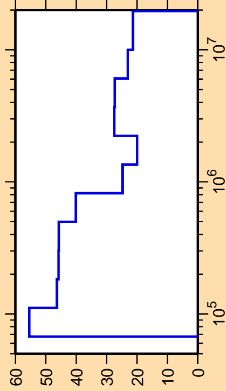
\Delta\sigma/\sigma vs. E for ^{181}\text{Os}(n,n_2)
