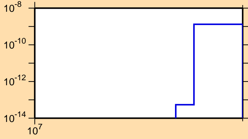
\sigma vs. E for ^{181}\text{Os}(n,nt)
