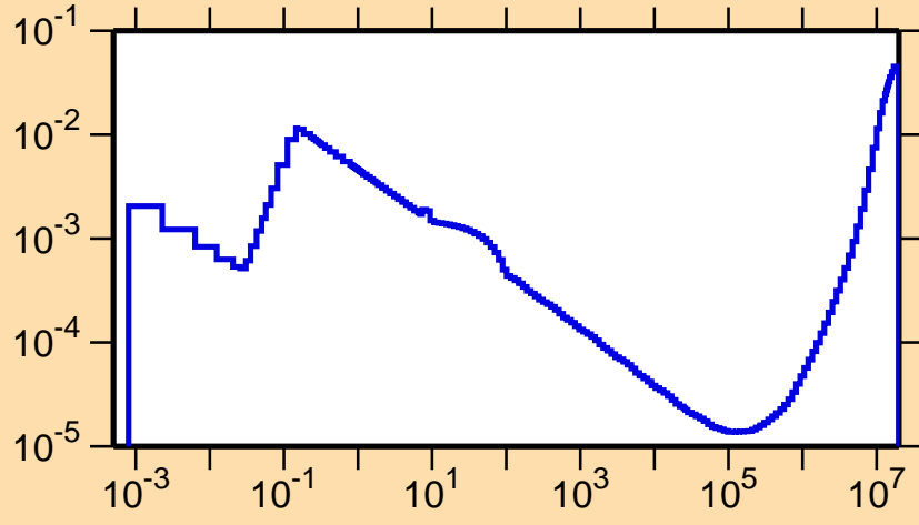
\sigma vs. E for ^{181}\text{Os}(n,p)
