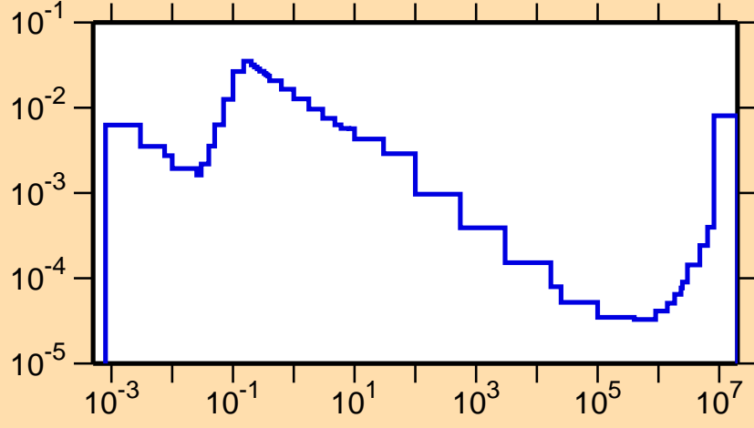
\sigma vs. E for ^{181}\text{Os}(n,\alpha)
