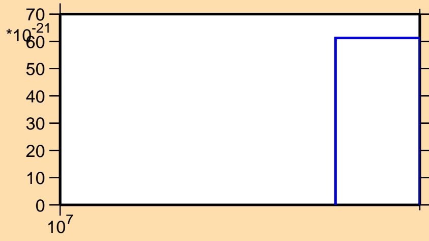
\sigma vs. E for ^{182}\text{Os} (mt 11)
