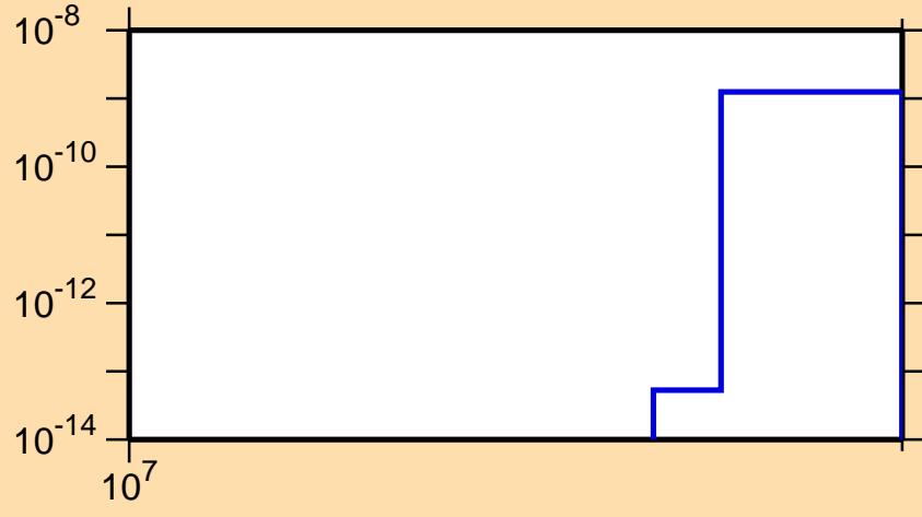
\sigma vs. E for ^{182}\text{Os}(n,nt)
