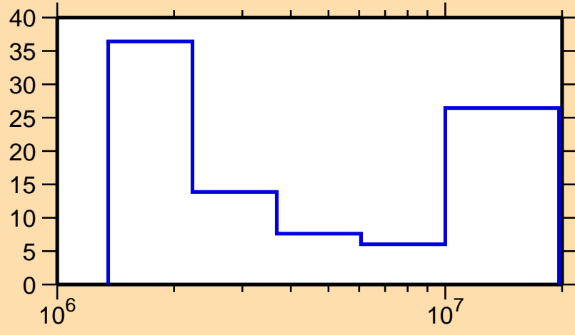
\Delta\sigma/\sigma vs. E for ^{182}\text{Os}(n,n\text{cont.})
