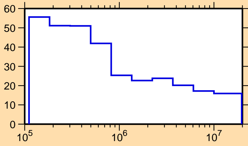
\Delta\sigma/\sigma vs. E for ^{182}\text{Os}(n,n_1)
