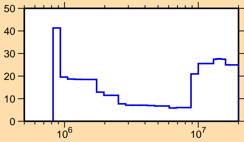
\Delta\sigma/\sigma vs. E for ^{183}\text{Os}(n,n\text{cont.})
