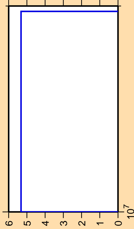
\Delta\sigma/\sigma vs. E for ^{183}\text{Os}(n,nt)
