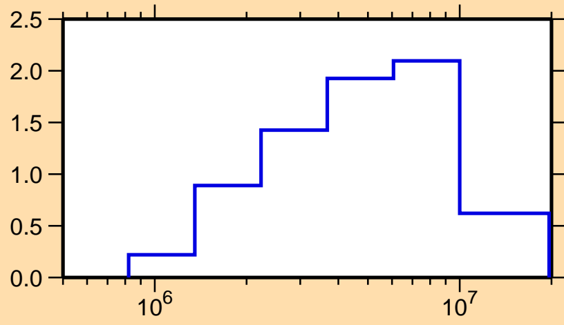
\sigma vs. E for ^{183}\text{Os}(n,n\text{cont.})
