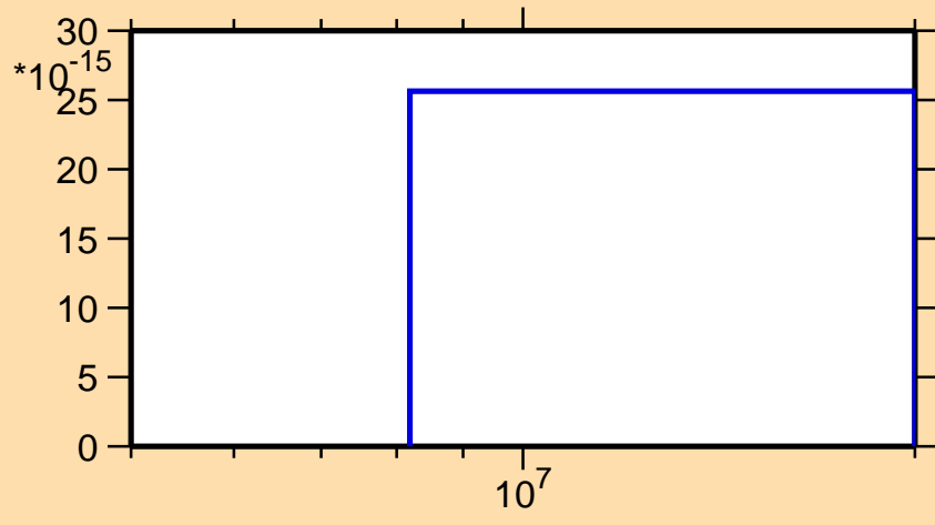
\sigma vs. E for ^{183}\text{Os}(n,pd)
