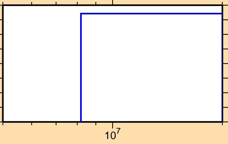
\sigma vs. E for ^{183}\text{Os}(n,\text{pt})
