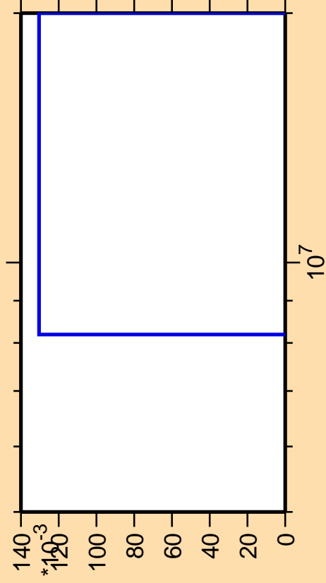
\Delta\sigma/\sigma vs. E for ^{183}\text{Os}(n,pd)
