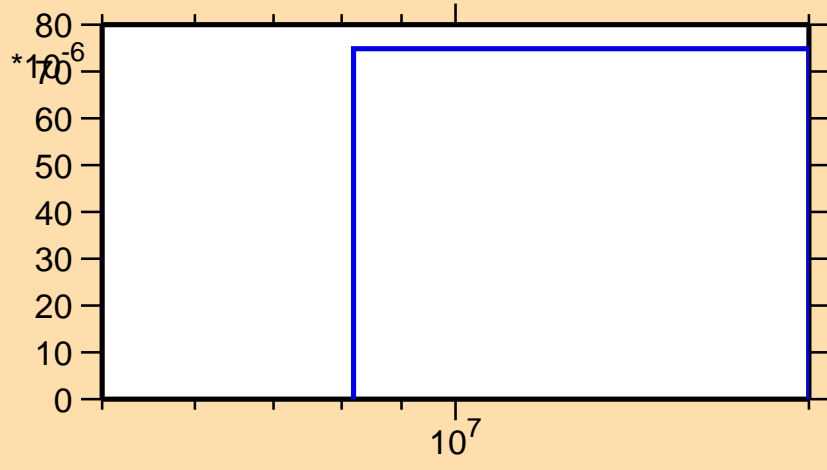
\sigma vs. E for ^{183}\text{Os}(n,t)
