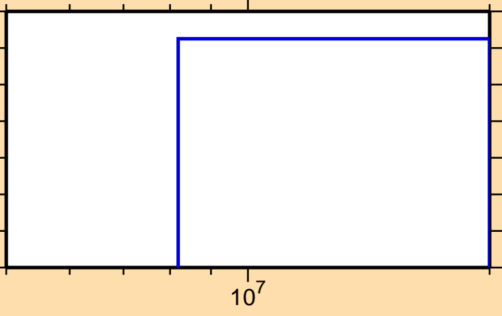
\sigma vs. E for ^{183}\text{Os}(\text{mt117})
