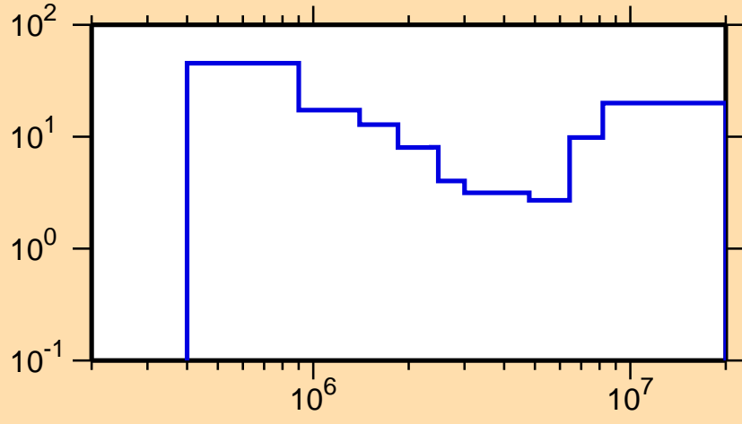
\Delta\sigma/\sigma vs. E for ^{183}\text{Os}(n,n\text{cont.})
