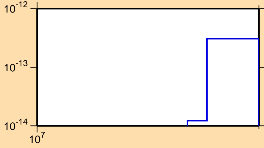
\sigma vs. E for ^{184}\text{Os}(\text{mt117})
