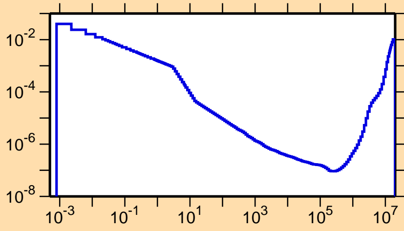
\sigma vs. E for ^{184}\text{Os}(n,\alpha)
