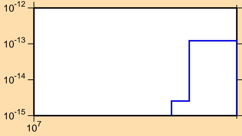
\sigma vs. E for ^{184}\text{Os} (mt 45)
