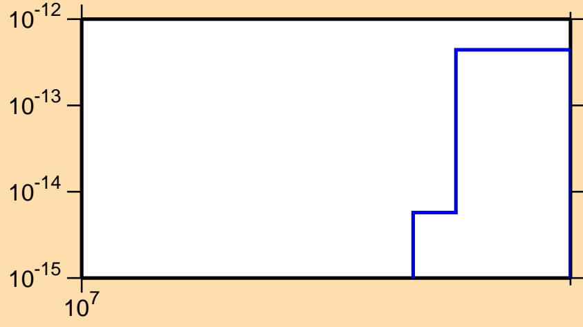
\sigma vs. E for ^{184}\text{Os}(n,\text{pd})
