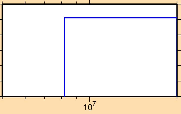
\sigma vs. E for ^{184}\text{Os}(n,2n\alpha)
