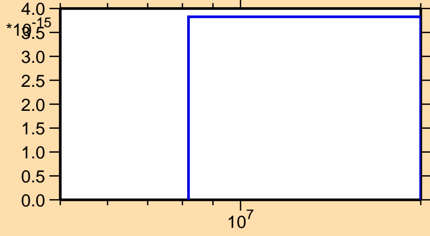
\sigma vs. E for ^{184}\text{Os}(n,pd)
