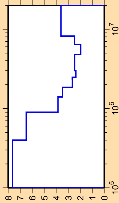
\Delta\sigma/\sigma vs. E for ^{184}\text{Os}(n,\text{inel.})
