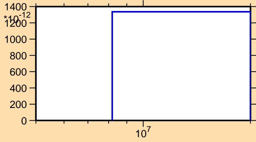
\sigma vs. E for ^{184}\text{Os}(n,nd)
