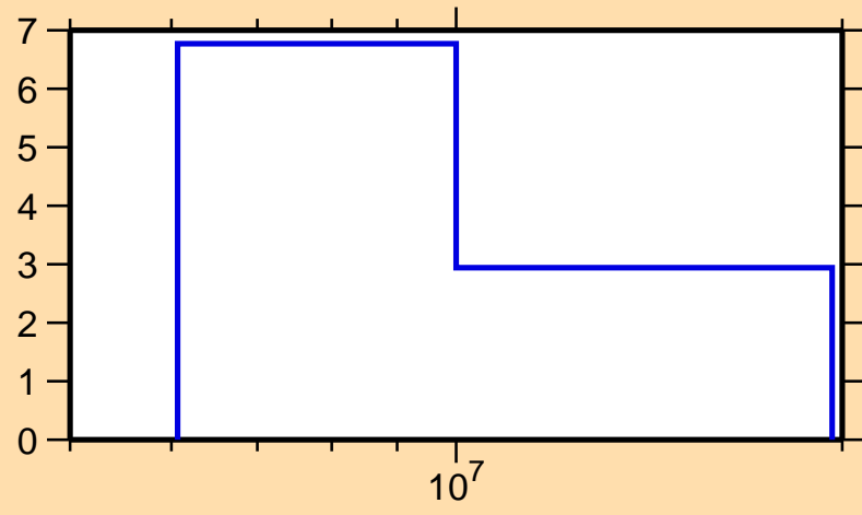
\Delta\sigma/\sigma vs. E for ^{185}\text{Os}(n,2n)
