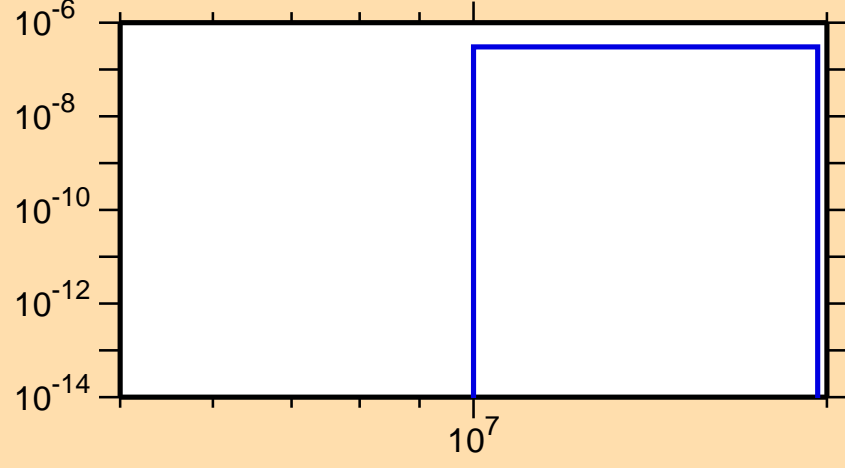
\sigma vs. E for ^{185}\text{Os}(n,2n\alpha)
