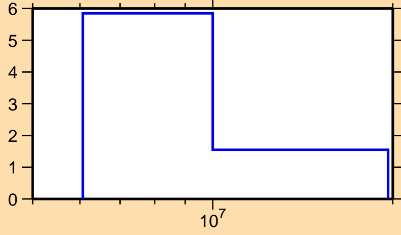
\Delta\sigma/\sigma vs. E for ^{185}\text{Os}(n,\text{el.})
