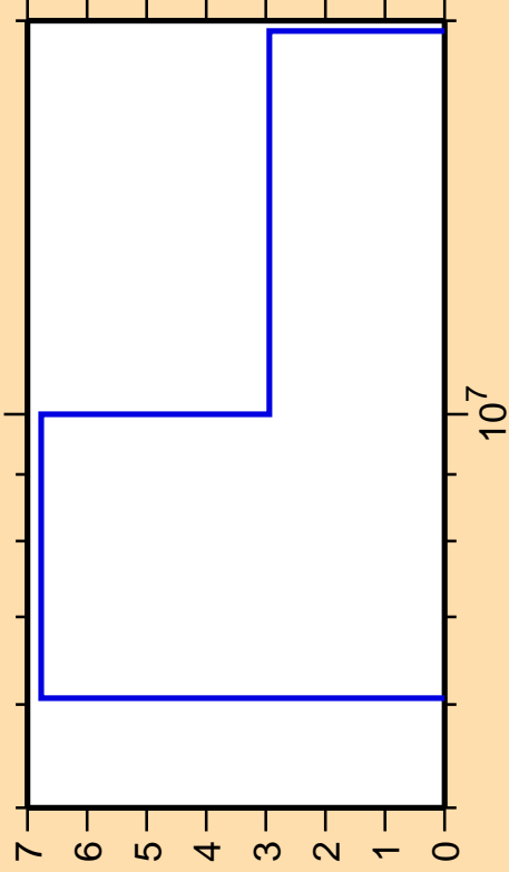
\Delta\sigma/\sigma vs. E for ^{185}\text{Os}(n,2n)
