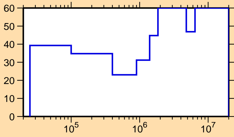
\Delta\sigma/\sigma vs. E for ^{185}\text{Os}(n,n_1)
