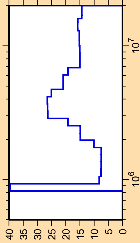
\Delta\sigma/\sigma vs. E for ^{186}\text{Os}(n,n_4)
