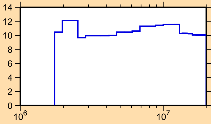
\Delta\sigma/\sigma vs. E for ^{186}\text{Os}(n, n_1)
