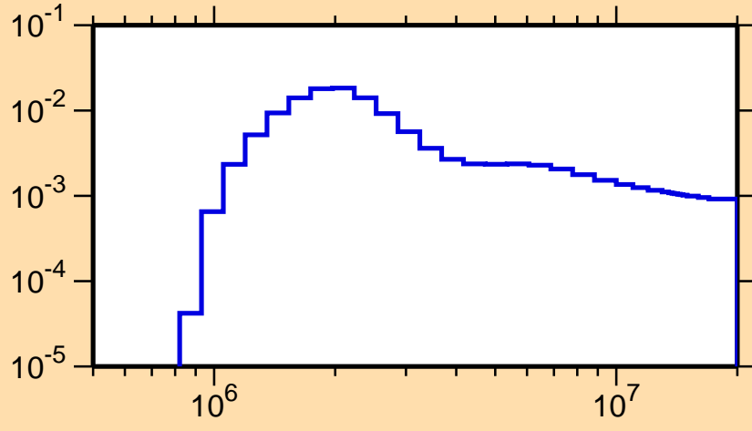
\sigma vs. E for ^{186}\text{Os}(n,n_4)
