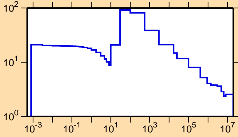
\sigma vs. E for ^{186}\text{Os}(n,\text{el.})
