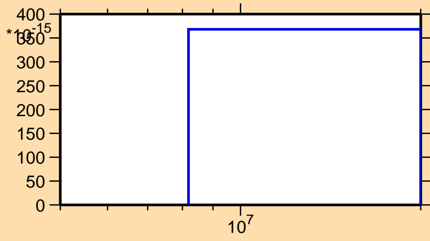
\sigma vs. E for ^{186}\text{Os}(n,p\alpha)
