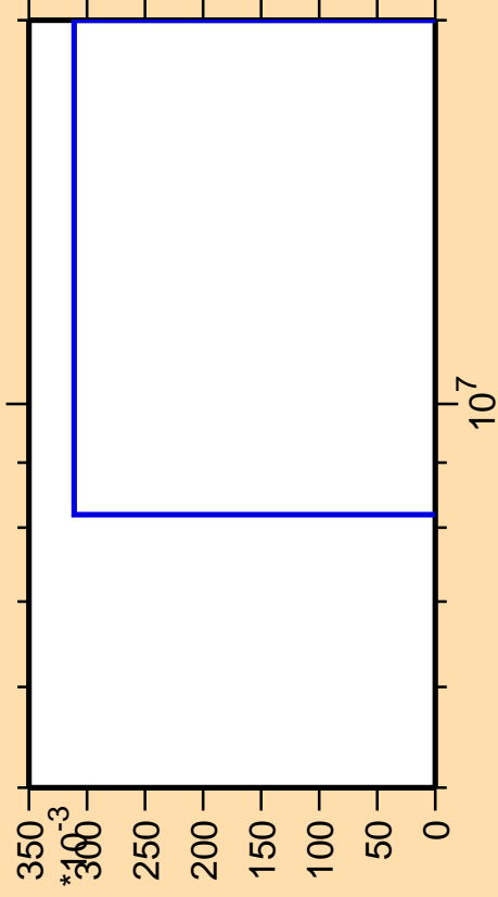
\Delta\sigma/\sigma vs. E for ^{186}\text{Os}(n,p\alpha)
