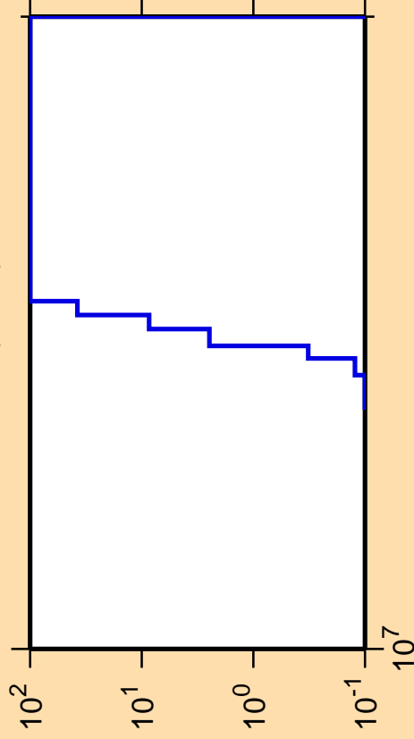
\Delta\sigma/\sigma vs. E for ^{187}\text{Os}(n,nd)
