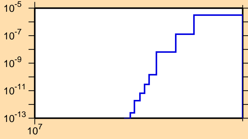
\sigma vs. E for ^{187}\text{Os}(n,nd)
