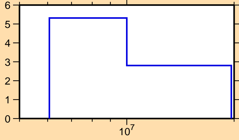
\Delta\sigma/\sigma vs. E for ^{187}\text{Os}(n,2n)
