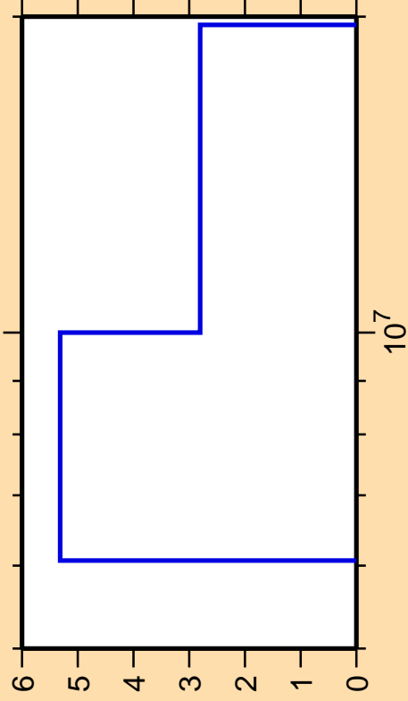
\Delta\sigma/\sigma vs. E for ^{187}\text{Os}(n,2n)
