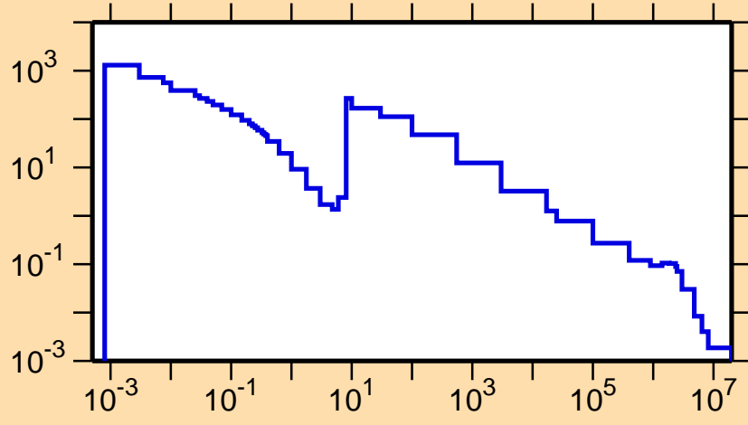
\sigma vs. E for ^{187}\text{Os}(n,\gamma)
