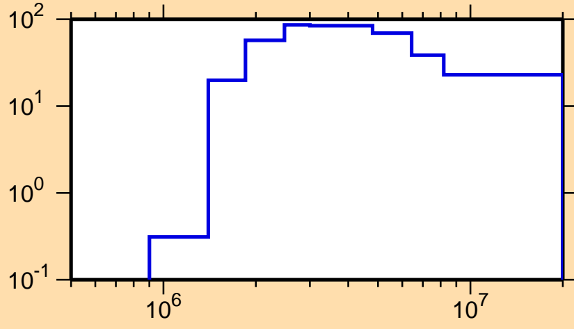
\Delta\sigma/\sigma vs. E for ^{187}\text{Os}(n,p)
