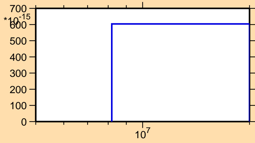
\sigma vs. E for ^{187}\text{Os}(n,p\alpha)
