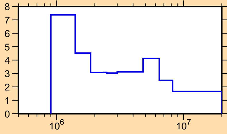
\Delta\sigma/\sigma vs. E for ^{187}\text{Os}(n,\text{el.})
