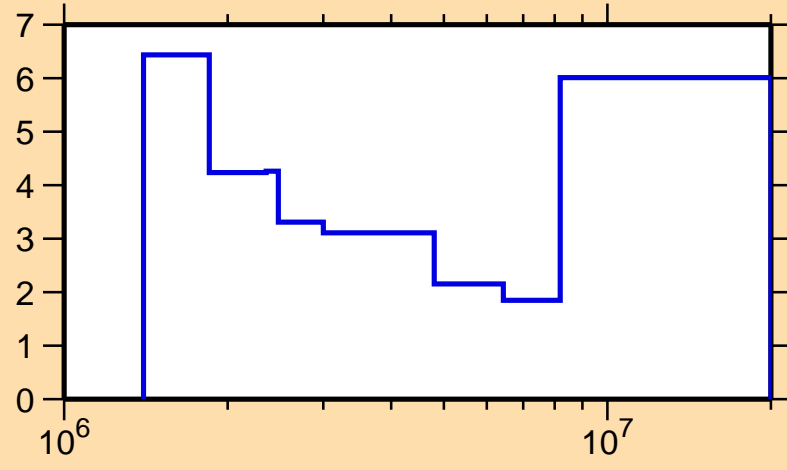
\Delta\sigma/\sigma vs. E for ^{188}\text{Os}(n,\text{inel.})
