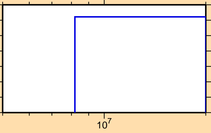
\sigma vs. E for ^{188}\text{Os}(n,t)
