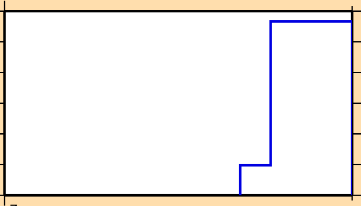
\sigma vs. E for ^{189}\text{Os}(n,p\alpha)
