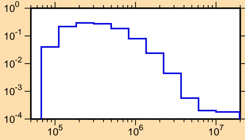
\sigma vs. E for ^{189}\text{Os}(n,n_4)
