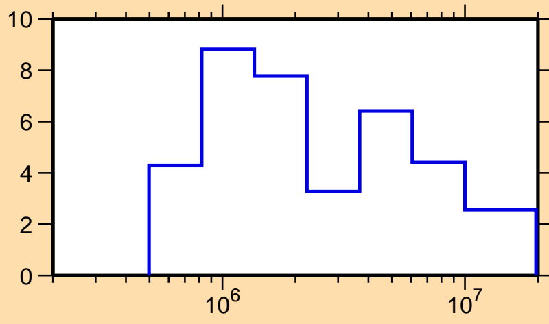
\Delta\sigma/\sigma vs. E for ^{189}\text{Os}(n, el.)
