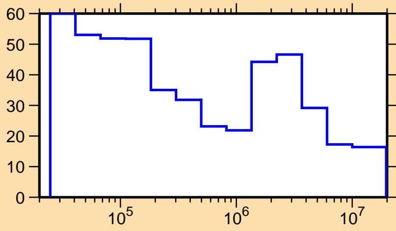
\Delta\sigma/\sigma vs. E for ^{189}\text{Os}(n,n_1)
