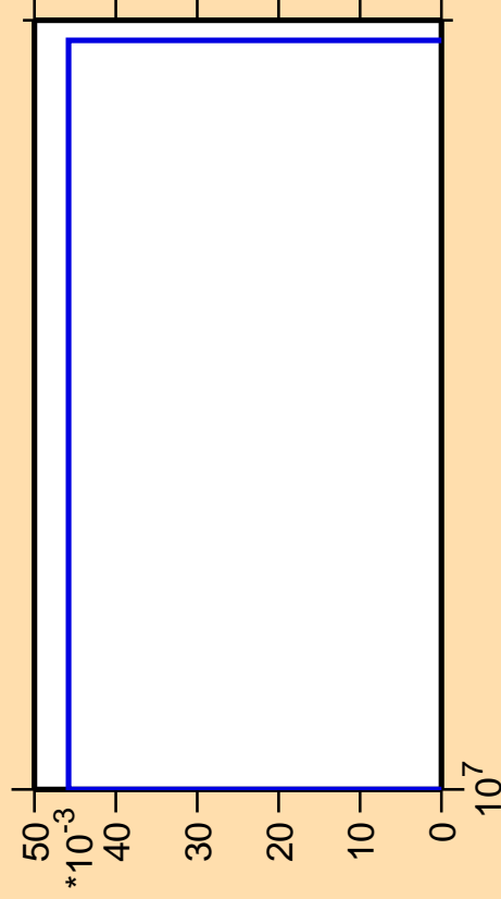
\Delta\sigma/\sigma vs. E for ^{189}\text{Os}(n,p\alpha)
