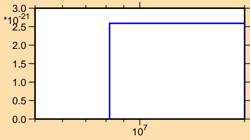
\sigma vs. E for ^{189}\text{Os} (mt 11)
