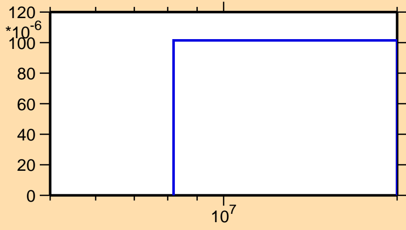
\sigma vs. E for ^{189}\text{Os}(n,t)
