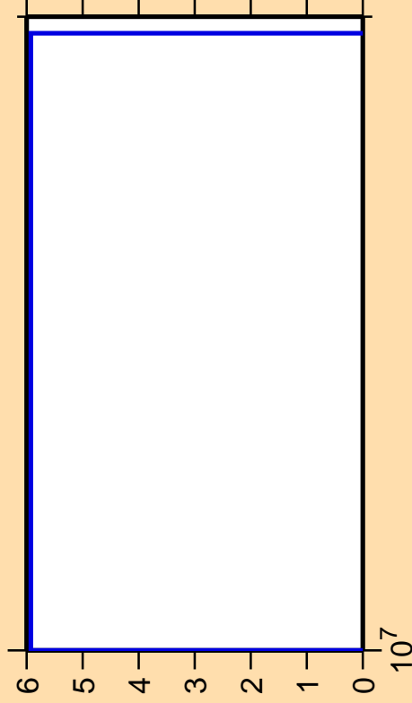
\Delta\sigma/\sigma vs. E for ^{189}\text{Os}(n,3n)
