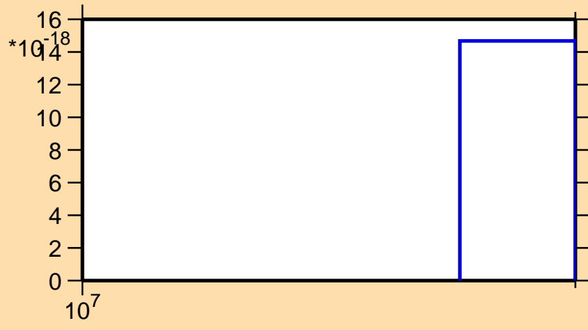
\sigma vs. E for ^{190}\text{Os} (mt 11)
