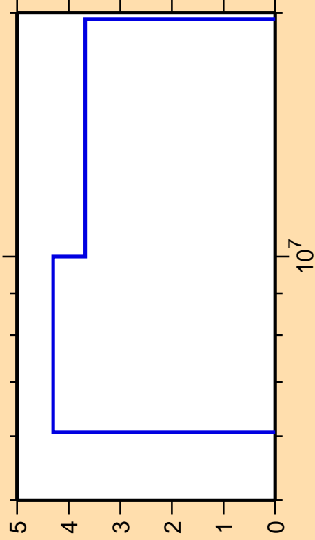
\Delta\sigma/\sigma vs. E for ^{190}\text{Os}(n,2n)
